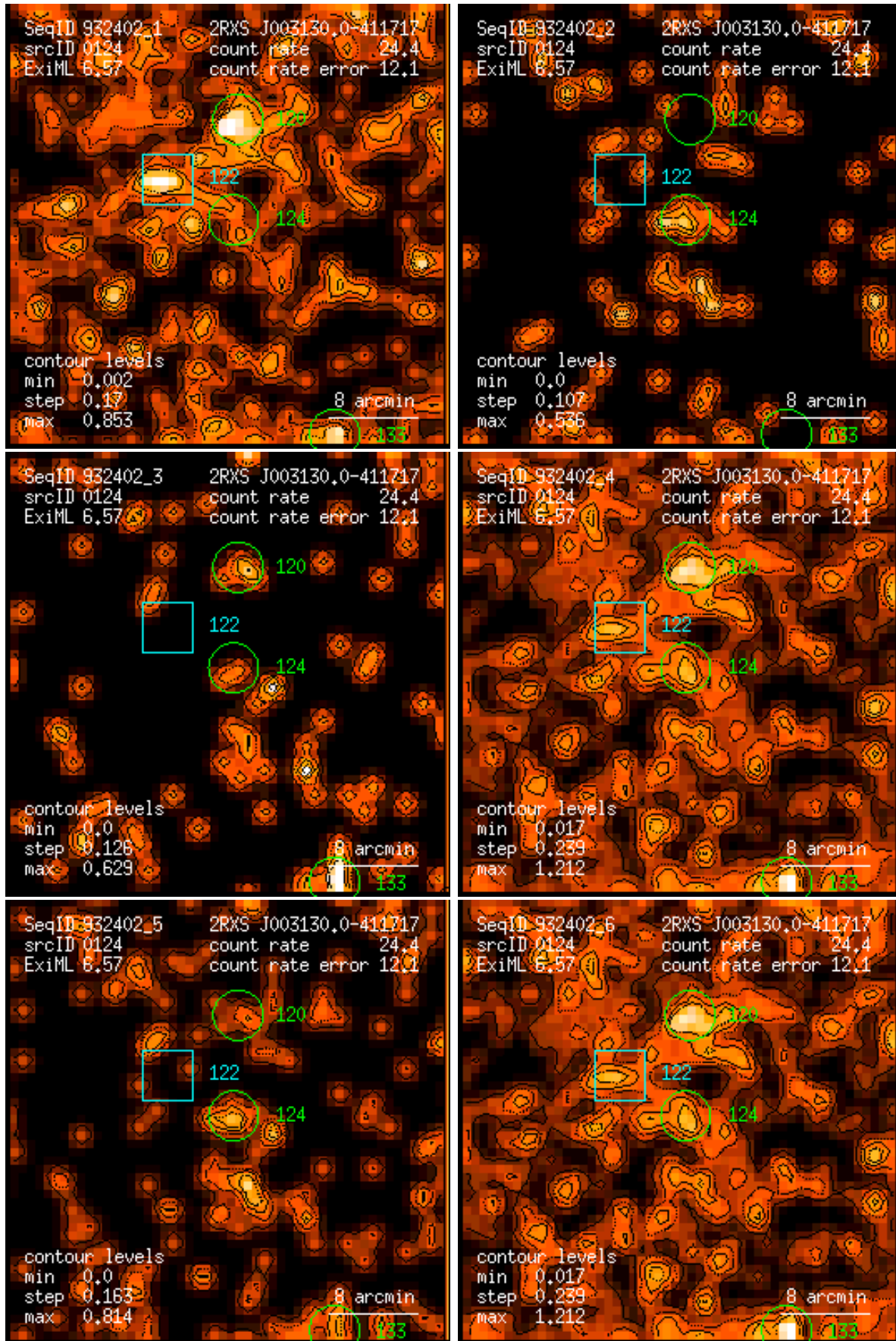
Figure 124: RASS 932402: detection 0124: band rate images, Gaussian filter: (1) PSPC channels 11 – 41, (2) 52 – 90, (3) 91 – 201, (4) 11 – 235, (5) 52 – 201, (6) 11 – 201. Broad band rates in counts/ks. Band rate contour levels in counts/ks/arcmin 2 .
