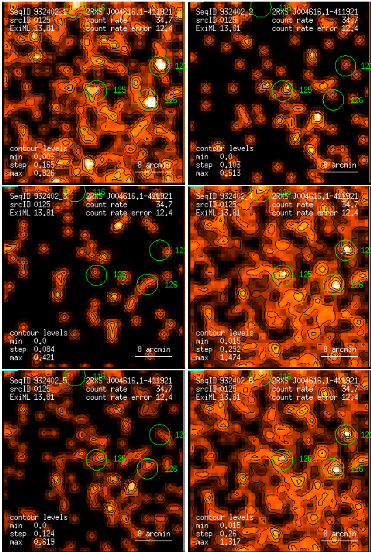
Figure 125: RASS 932402: detection 0125: band rate images, Gaussian filter: (1) PSPC channels 11 – 41, (2) 52 – 90, (3) 91 – 201, (4) 11 – 235, (5) 52 – 201, (6) 11 – 201. Broad band rates in counts/ks. Band rate contour levels in counts/ks/arcmin 2 .
