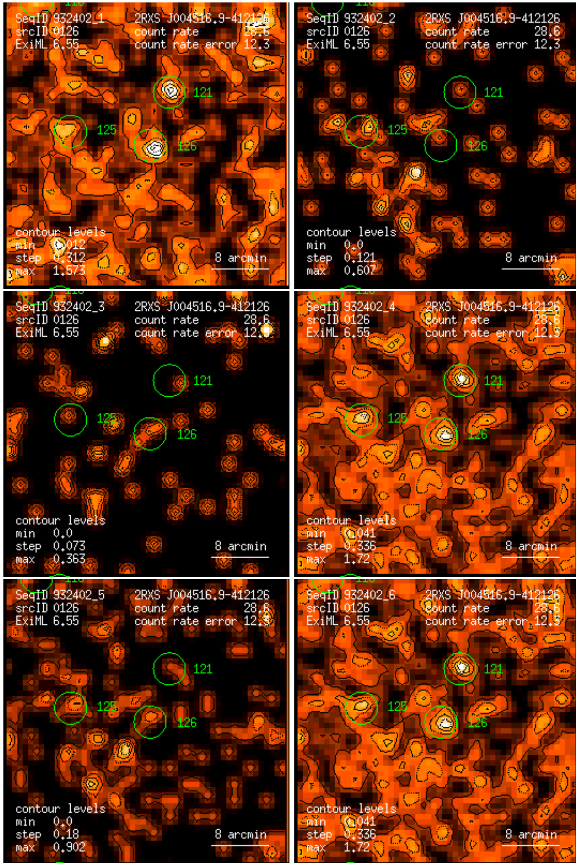
Figure 126: RASS 932402: detection 0126: band rate images, Gaussian filter: (1) PSPC channels 11 – 41, (2) 52 – 90, (3) 91 – 201, (4) 11 – 235, (5) 52 – 201, (6) 11 – 201. Broad band rates in counts/ks. Band rate contour levels in counts/ks/arcmin 2 .
