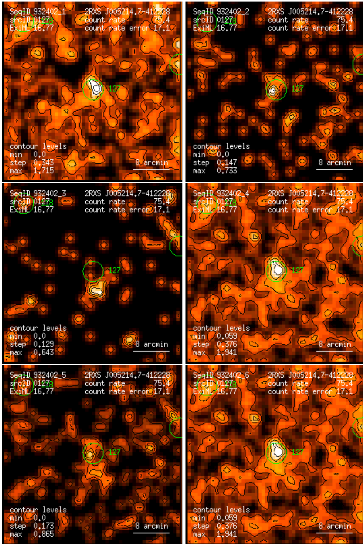
Figure 127: RASS 932402: detection 0127: band rate images, Gaussian filter: (1) PSPC channels 11 – 41, (2) 52 – 90, (3) 91 – 201, (4) 11 – 235, (5) 52 – 201, (6) 11 – 201. Broad band rates in counts/ks. Band rate contour levels in counts/ks/arcmin 2 .
