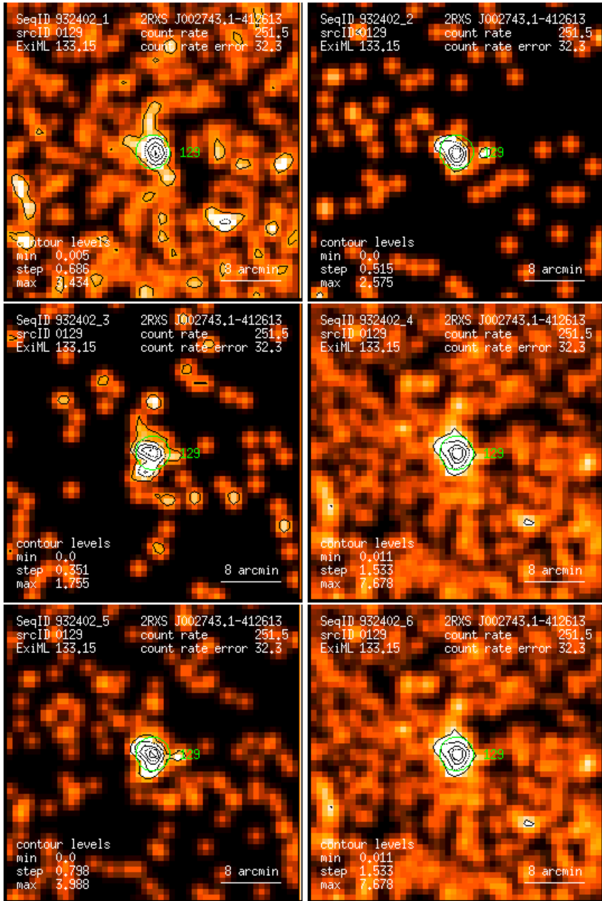
Figure 129: RASS 932402: detection 0129: band rate images, Gaussian filter: (1) PSPC channels 11 – 41, (2) 52 – 90, (3) 91 – 201, (4) 11 – 235, (5) 52 – 201, (6) 11 – 201. Broad band rates in counts/ks. Band rate contour levels in counts/ks/arcmin 2 .
