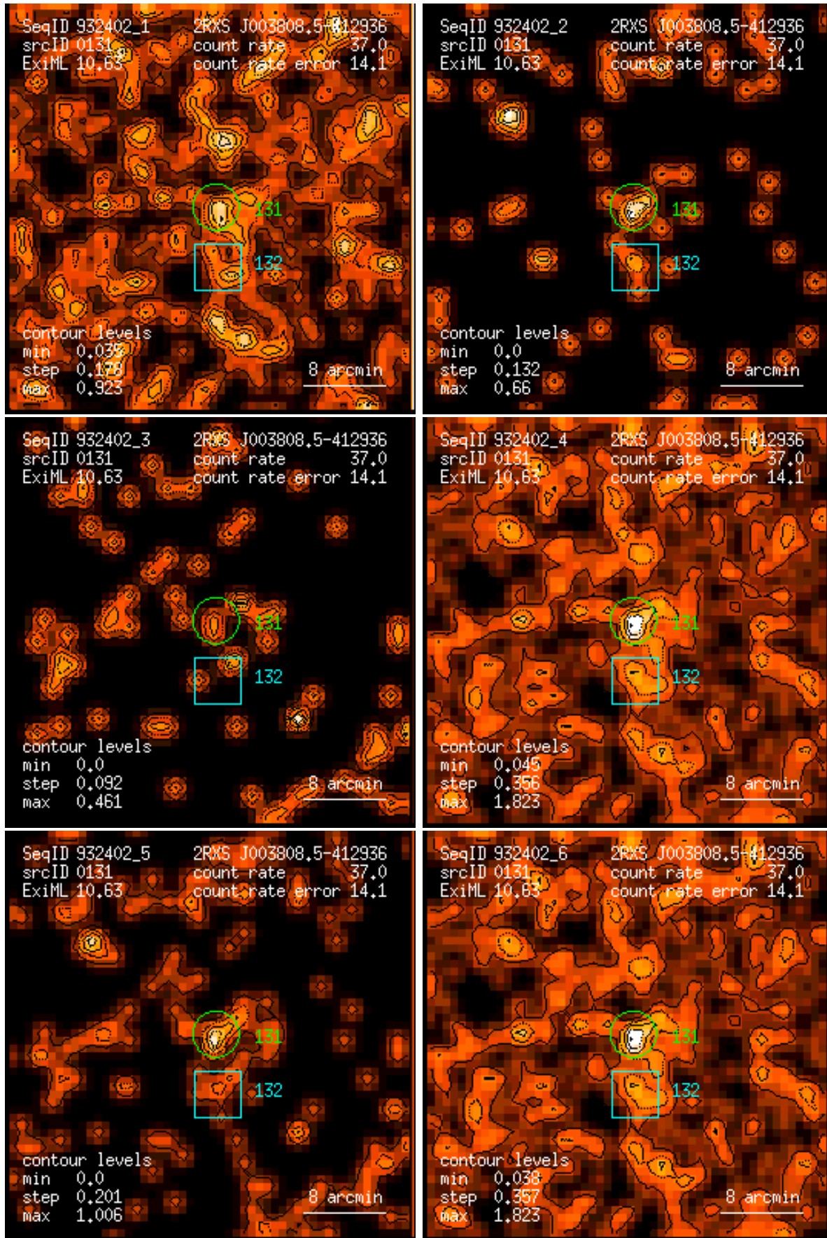
Figure 131: RASS 932402: detection 0131: band rate images, Gaussian filter: (1) PSPC channels 11 – 41, (2) 52 – 90, (3) 91 – 201, (4) 11 – 235, (5) 52 – 201, (6) 11 – 201. Broad band rates in counts/ks. Band rate contour levels in counts/ks/arcmin 2 .
