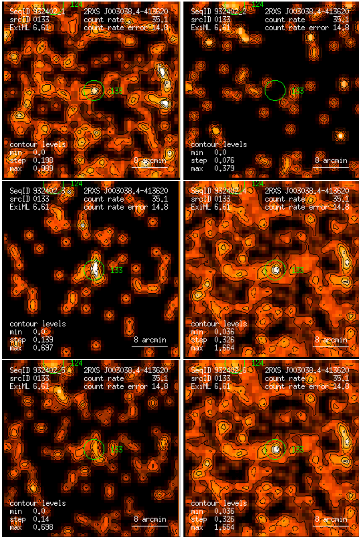
Figure 133: RASS 932402: detection 0133: band rate images, Gaussian filter: (1) PSPC channels 11 – 41, (2) 52 – 90, (3) 91 – 201, (4) 11 – 235, (5) 52 – 201, (6) 11 – 201. Broad band rates in counts/ks. Band rate contour levels in counts/ks/arcmin 2 .
