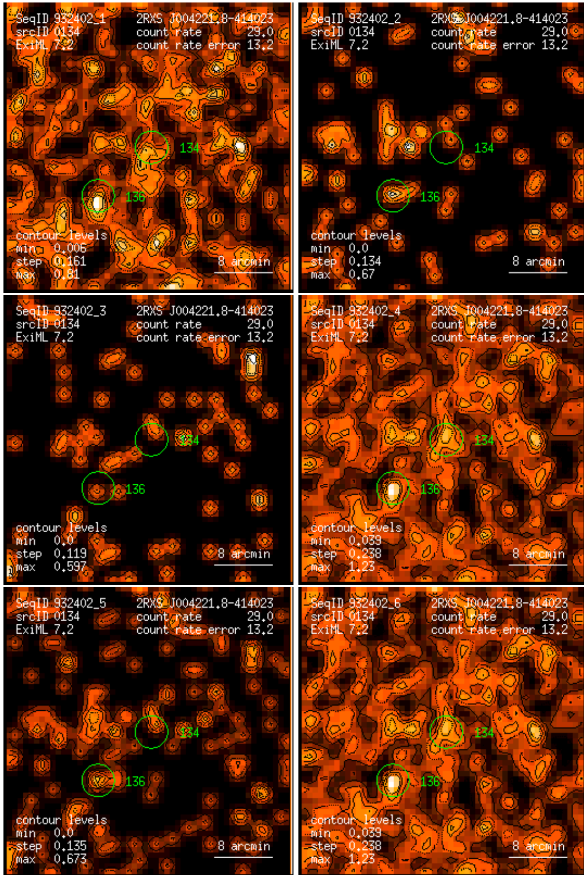
Figure 134: RASS 932402: detection 0134: band rate images, Gaussian filter: (1) PSPC channels 11 – 41, (2) 52 – 90, (3) 91 – 201, (4) 11 – 235, (5) 52 – 201, (6) 11 – 201. Broad band rates in counts/ks. Band rate contour levels in counts/ks/arcmin 2 .
