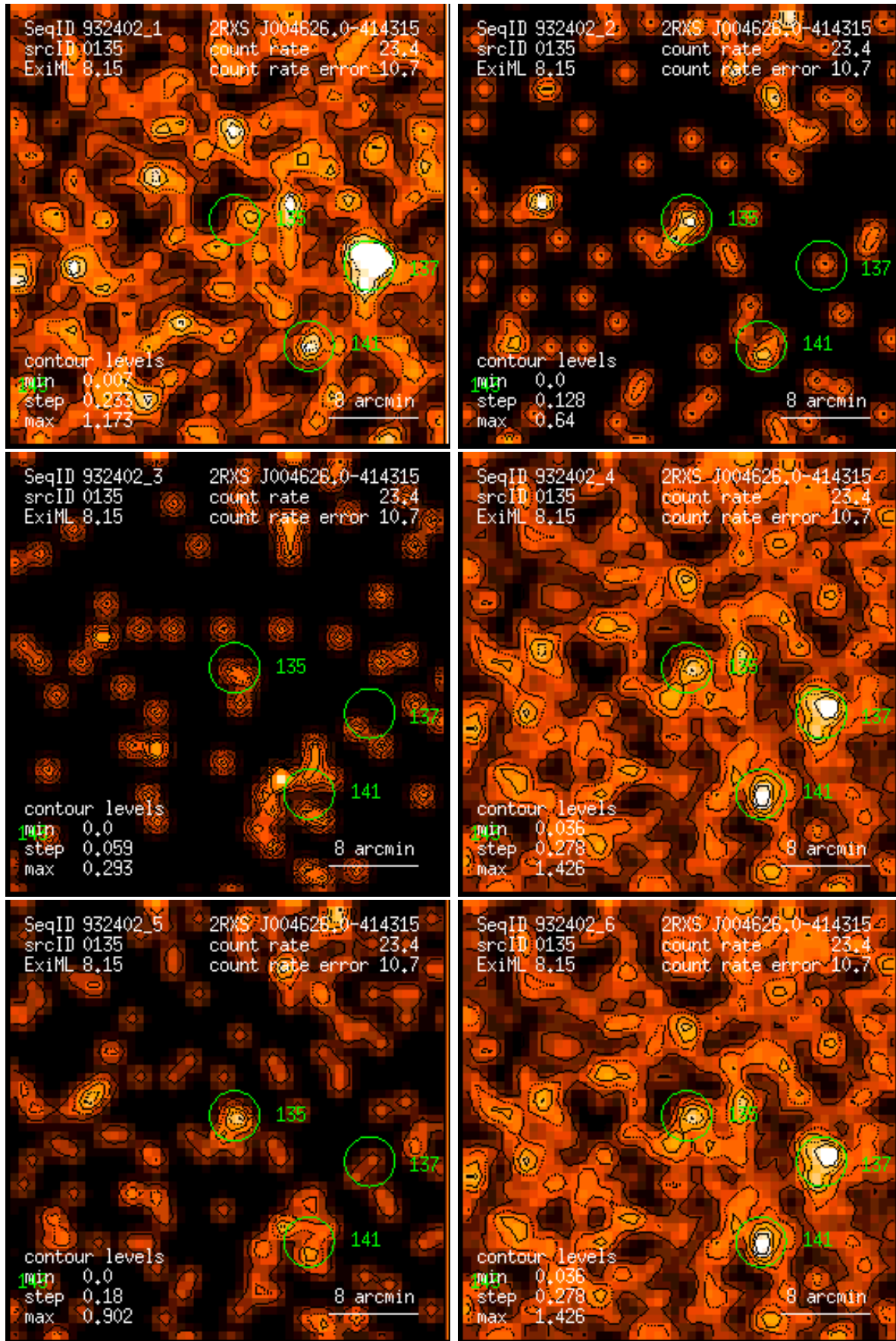
Figure 135: RASS 932402: detection 0135: band rate images, Gaussian filter: (1) PSPC channels 11 – 41, (2) 52 – 90, (3) 91 – 201, (4) 11 – 235, (5) 52 – 201, (6) 11 – 201. Broad band rates in counts/ks. Band rate contour levels in counts/ks/arcmin 2 .
