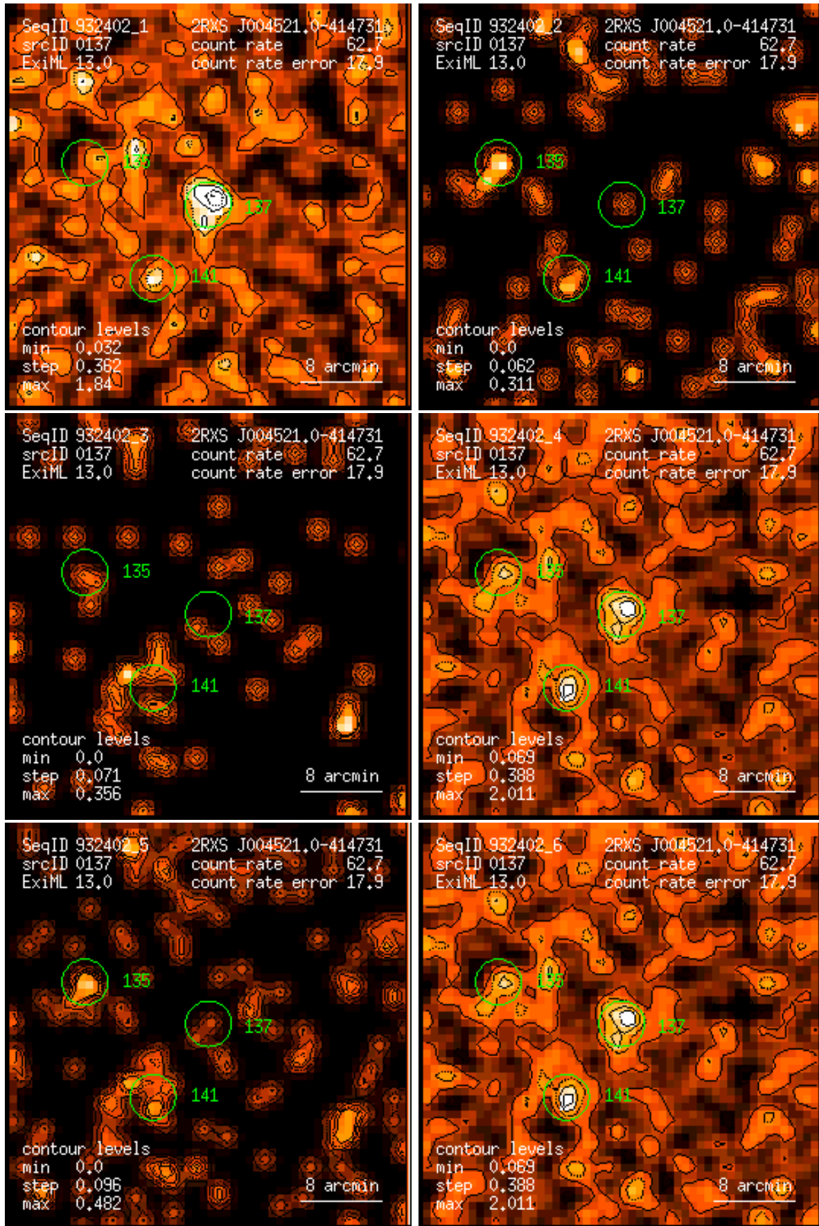
Figure 137: RASS 932402: detection 0137: band rate images, Gaussian filter: (1) PSPC channels 11 – 41, (2) 52 – 90, (3) 91 – 201, (4) 11 – 235, (5) 52 – 201, (6) 11 – 201. Broad band rates in counts/ks. Band rate contour levels in counts/ks/arcmin 2 .
