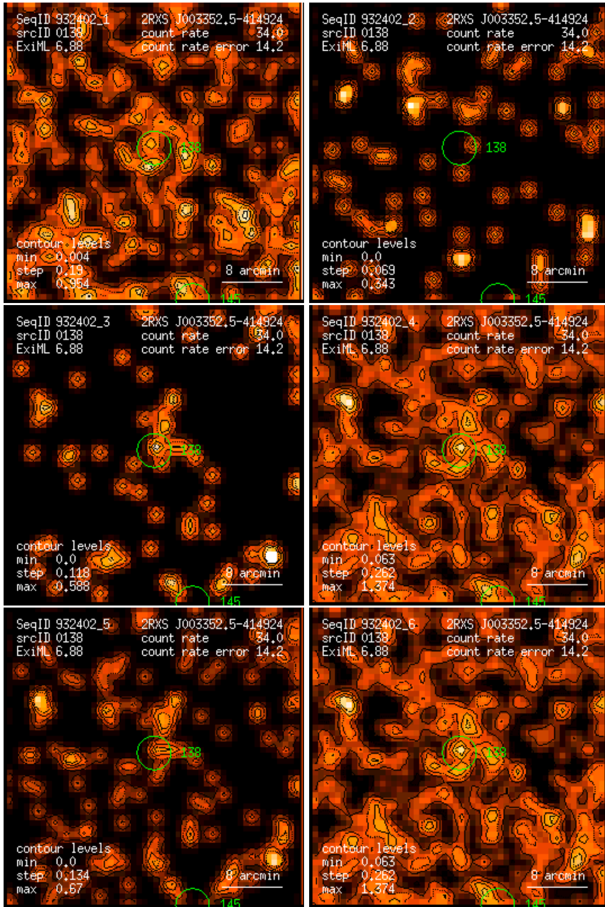
Figure 138: RASS 932402: detection 0138: band rate images, Gaussian filter: (1) PSPC channels 11 – 41, (2) 52 – 90, (3) 91 – 201, (4) 11 – 235, (5) 52 – 201, (6) 11 – 201. Broad band rates in counts/ks. Band rate contour levels in counts/ks/arcmin 2 .
