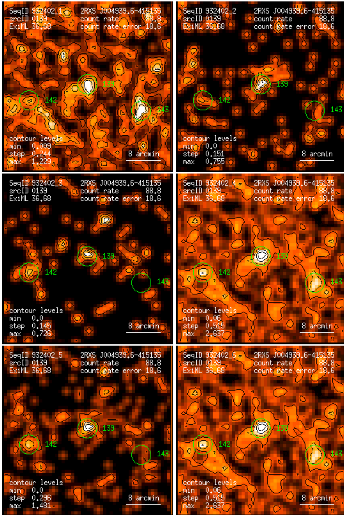
Figure 139: RASS 932402: detection 0139: band rate images, Gaussian filter: (1) PSPC channels 11 – 41, (2) 52 – 90, (3) 91 – 201, (4) 11 – 235, (5) 52 – 201, (6) 11 – 201. Broad band rates in counts/ks. Band rate contour levels in counts/ks/arcmin 2 .
