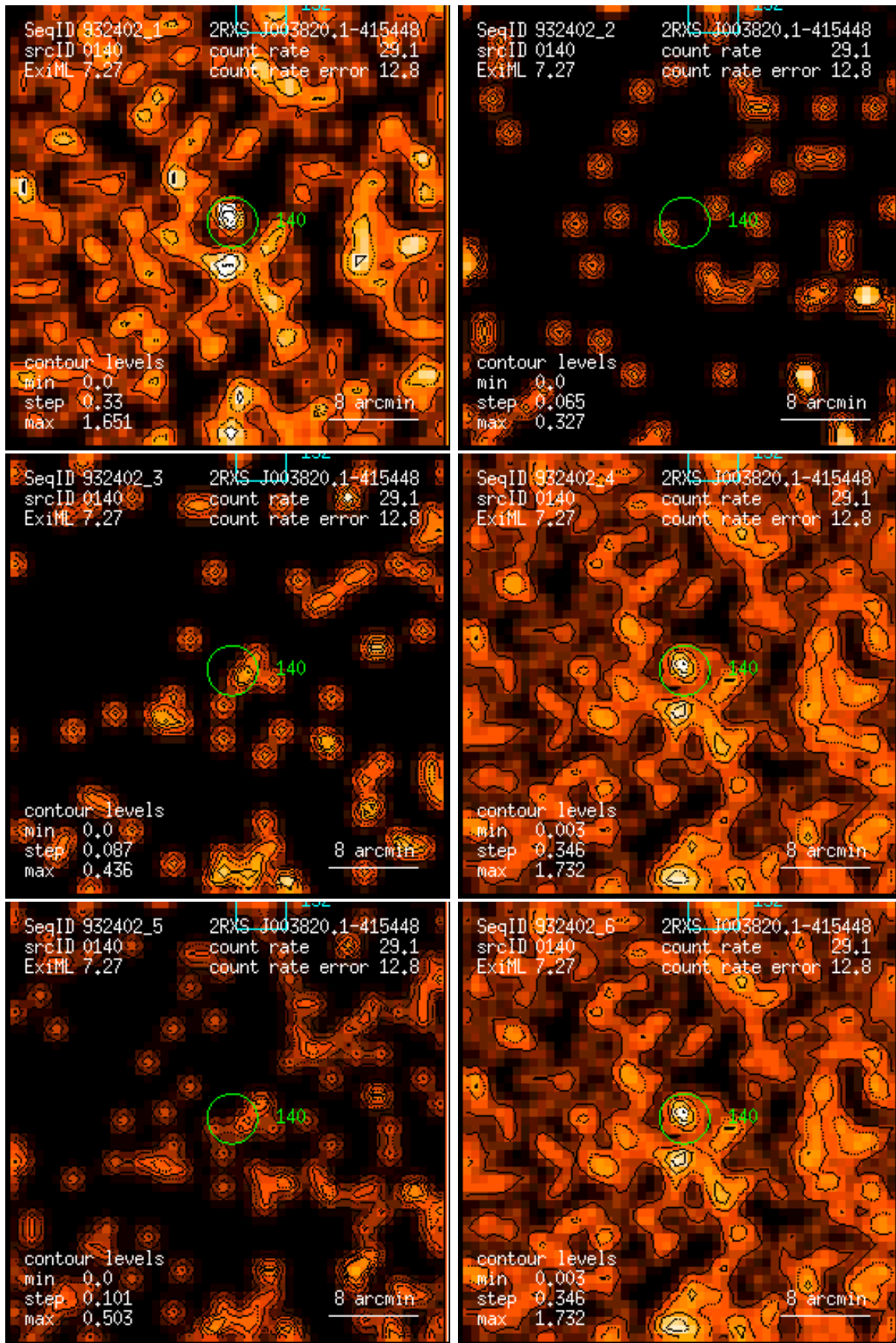
Figure 140: RASS 932402: detection 0140: band rate images, Gaussian filter: (1) PSPC channels 11 – 41, (2) 52 – 90, (3) 91 – 201, (4) 11 – 235, (5) 52 – 201, (6) 11 – 201. Broad band rates in counts/ks. Band rate contour levels in counts/ks/arcmin 2 .
