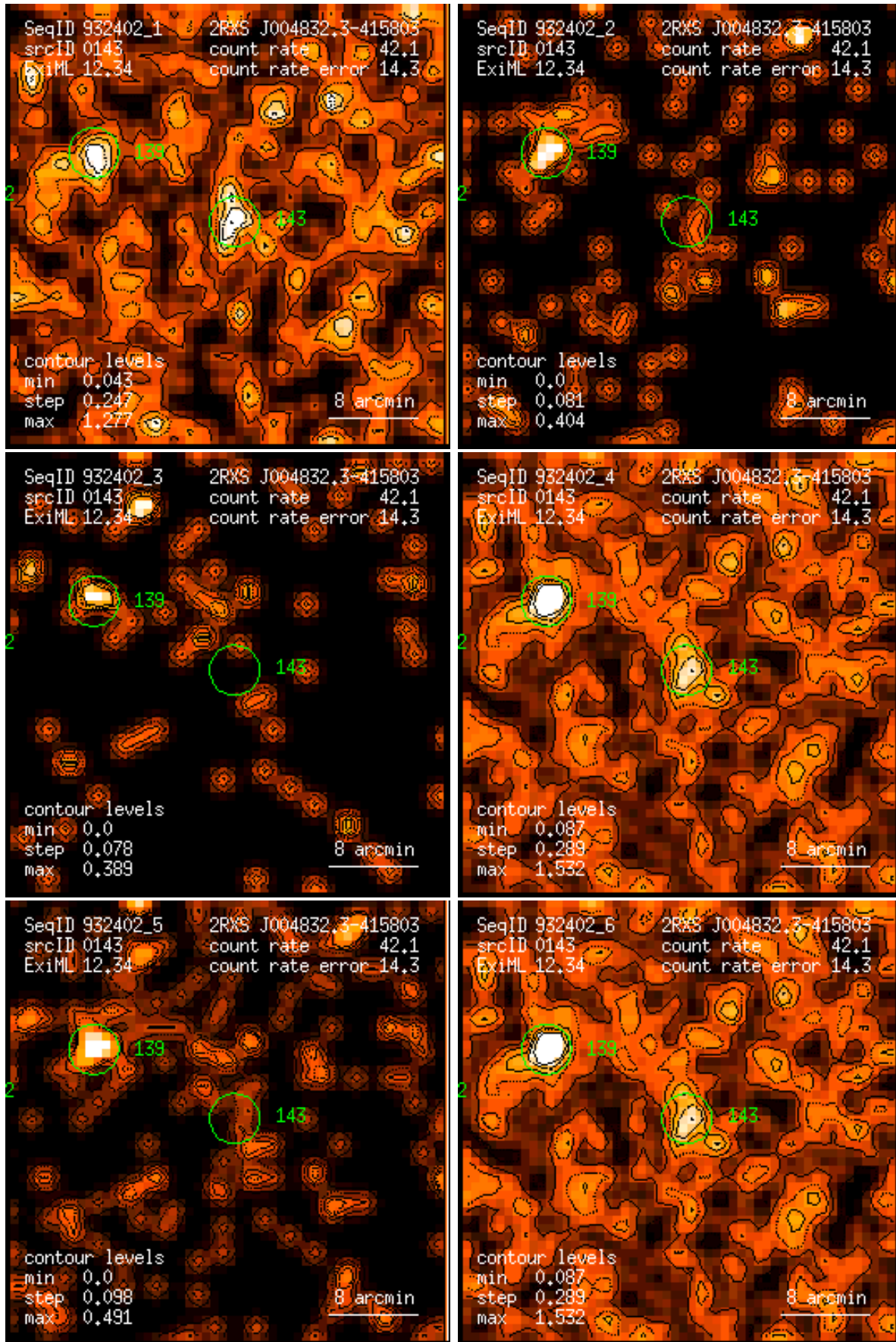
Figure 143: RASS 932402: detection 0143: band rate images, Gaussian filter: (1) PSPC channels 11 – 41, (2) 52 – 90, (3) 91 – 201, (4) 11 – 235, (5) 52 – 201, (6) 11 – 201. Broad band rates in counts/ks. Band rate contour levels in counts/ks/arcmin 2 .
