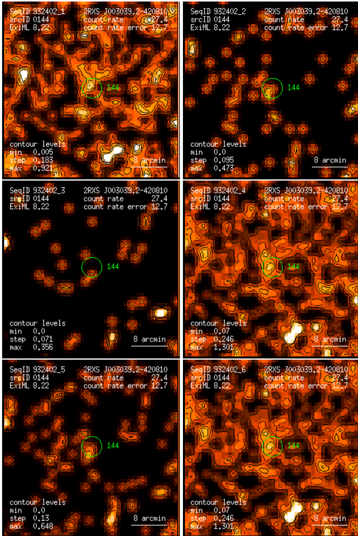
Figure 144: RASS 932402: detection 0144: band rate images, Gaussian filter: (1) PSPC channels 11 – 41, (2) 52 – 90, (3) 91 – 201, (4) 11 – 235, (5) 52 – 201, (6) 11 – 201. Broad band rates in counts/ks. Band rate contour levels in counts/ks/arcmin 2 .
