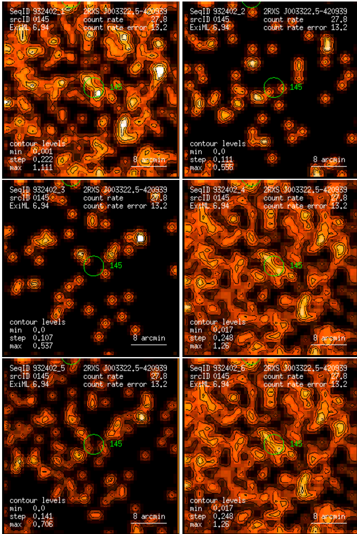
Figure 145: RASS 932402: detection 0145: band rate images, Gaussian filter: (1) PSPC channels 11 – 41, (2) 52 – 90, (3) 91 – 201, (4) 11 – 235, (5) 52 – 201, (6) 11 – 201. Broad band rates in counts/ks. Band rate contour levels in counts/ks/arcmin 2 .
