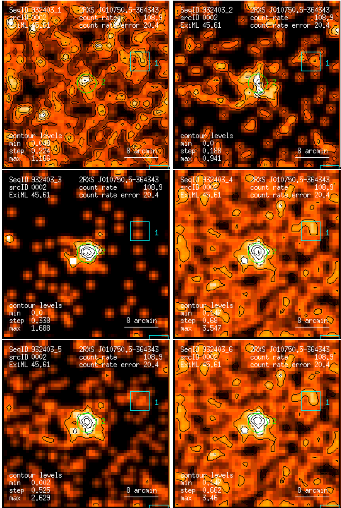
Figure 2: RASS 932403: detection 0002: band rate images, Gaussian filter: (1) PSPC channels 11 – 41, (2) 52 – 90, (3) 91 – 201, (4) 11 – 235, (5) 52 – 201, (6) 11 – 201. Broad band rates in counts/ks. Band rate contour levels in counts/ks/arcmin 2 .
