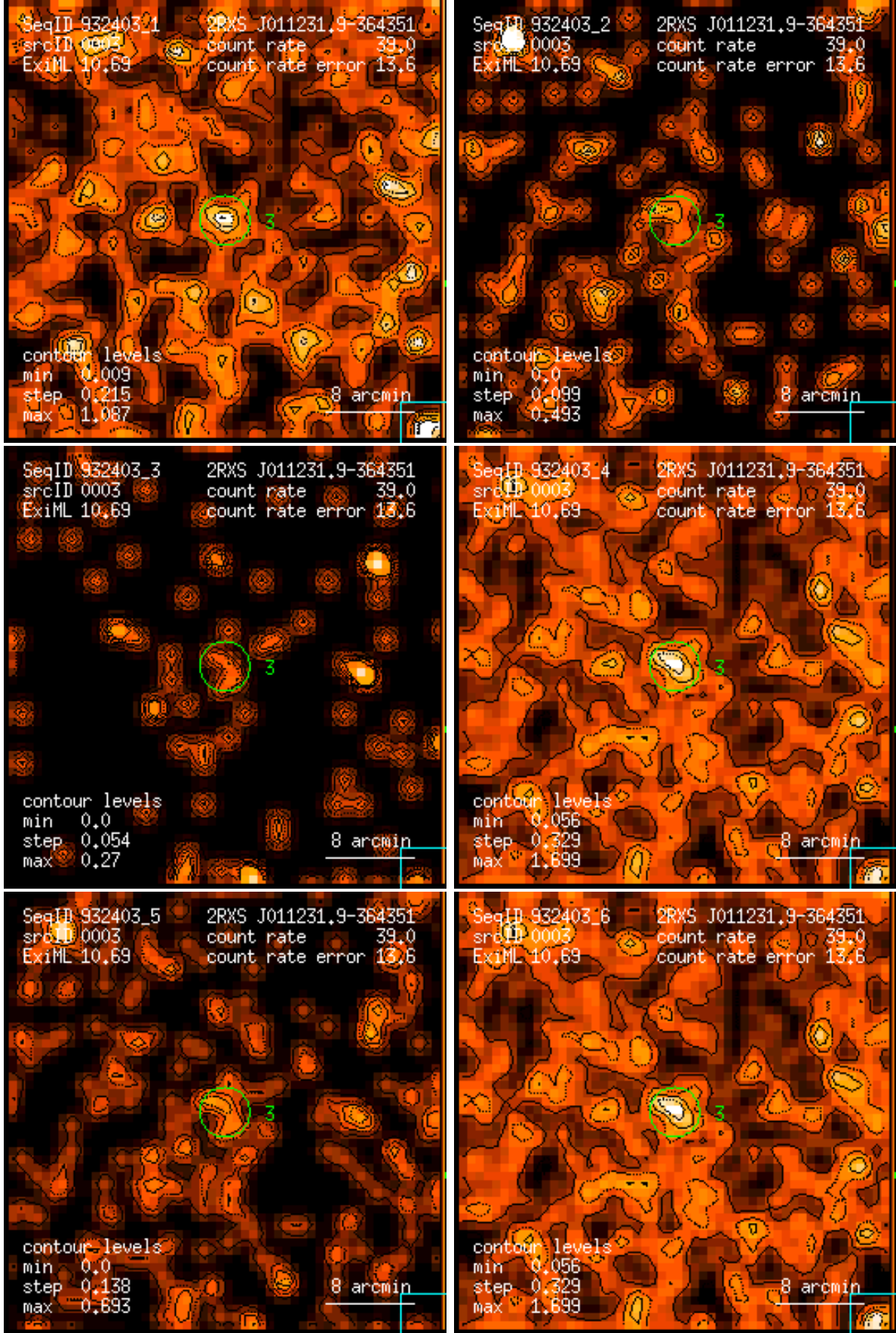
Figure 3: RASS 932403: detection 0003: band rate images, Gaussian filter: (1) PSPC channels 11 – 41, (2) 52 – 90, (3) 91 – 201, (4) 11 – 235, (5) 52 – 201, (6) 11 – 201. Broad band rates in counts/ks. Band rate contour levels in counts/ks/arcmin 2 .
