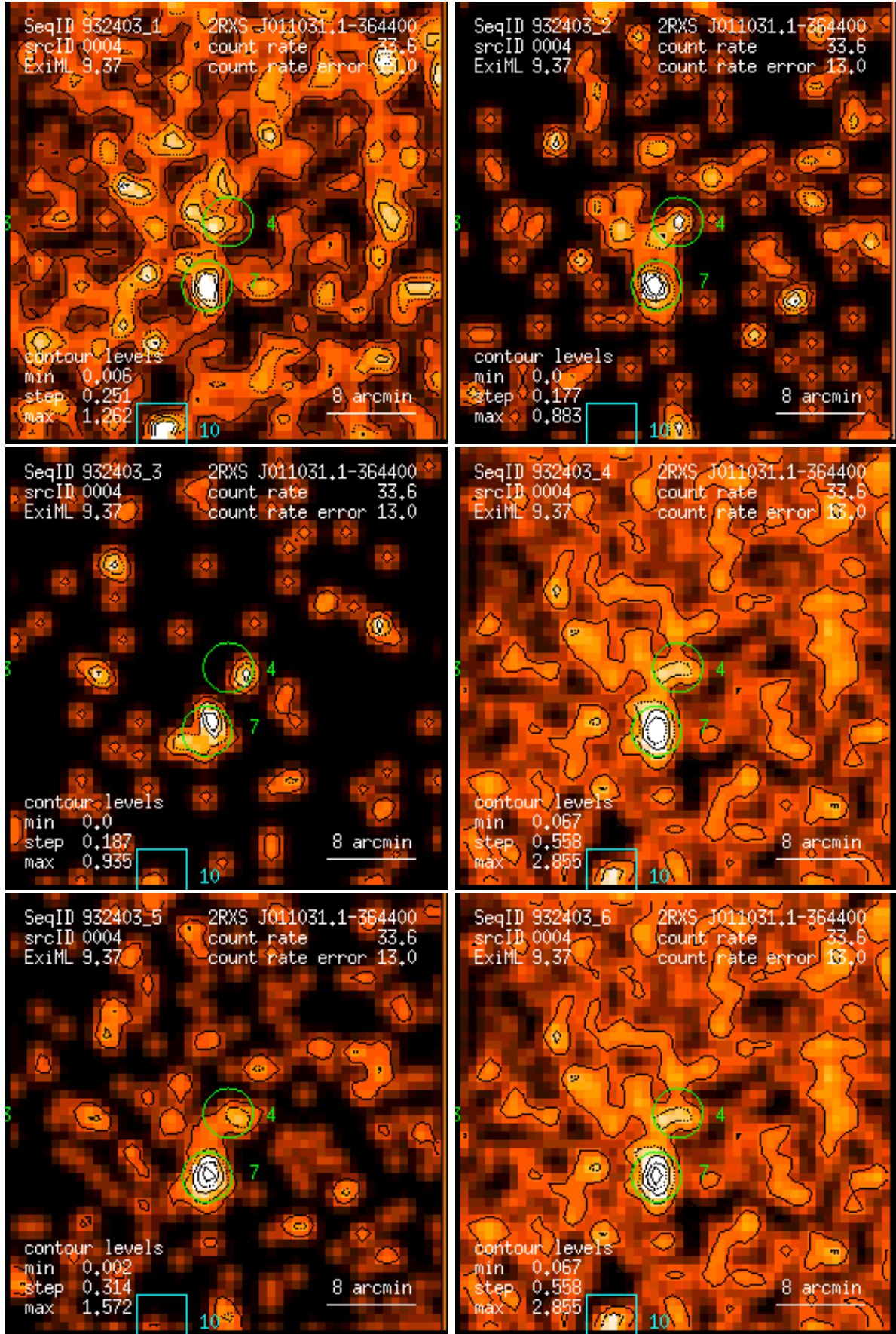
Figure 4: RASS 932403: detection 0004: band rate images, Gaussian filter: (1) PSPC channels 11 – 41, (2) 52 – 90, (3) 91 – 201, (4) 11 – 235, (5) 52 – 201, (6) 11 – 201. Broad band rates in counts/ks. Band rate contour levels in counts/ks/arcmin 2 .
