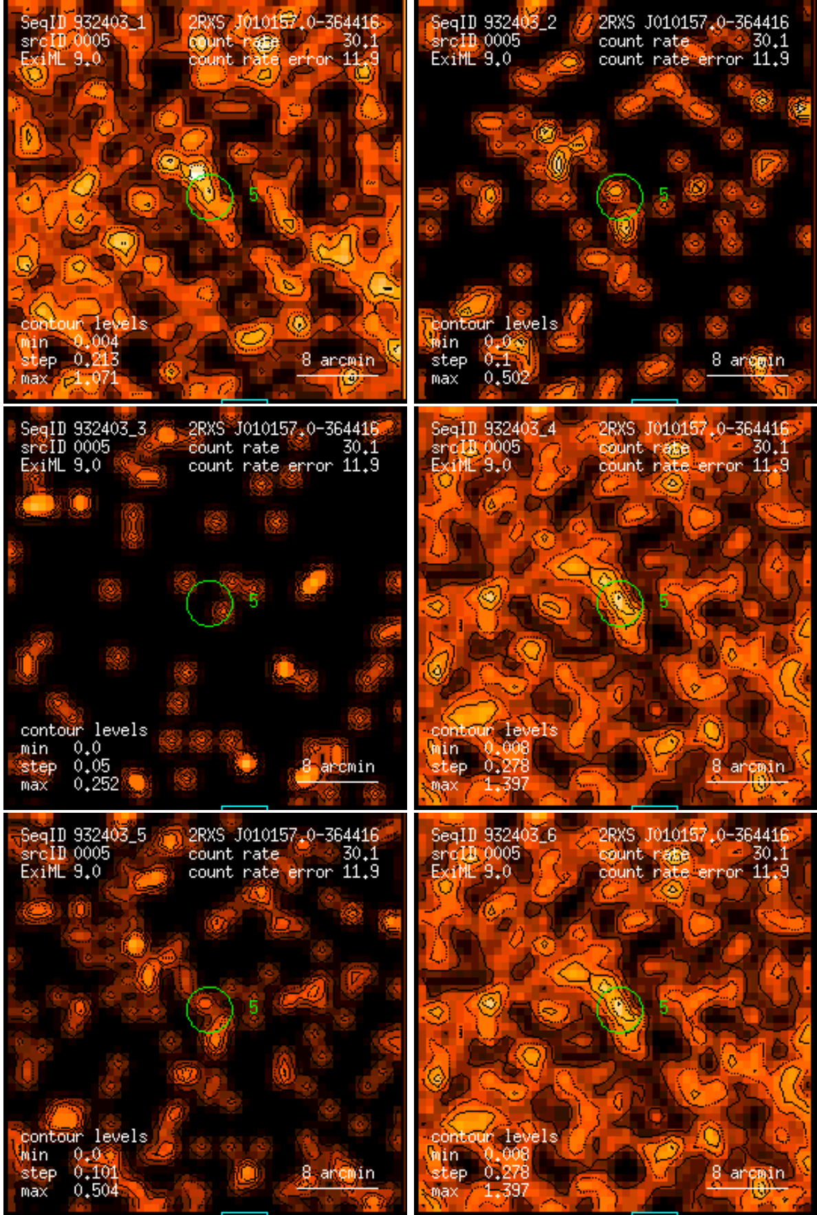
Figure 5: RASS 932403: detection 0005: band rate images, Gaussian filter: (1) PSPC channels 11 – 41, (2) 52 – 90, (3) 91 – 201, (4) 11 – 235, (5) 52 – 201, (6) 11 – 201. Broad band rates in counts/ks. Band rate contour levels in counts/ks/arcmin 2 .
