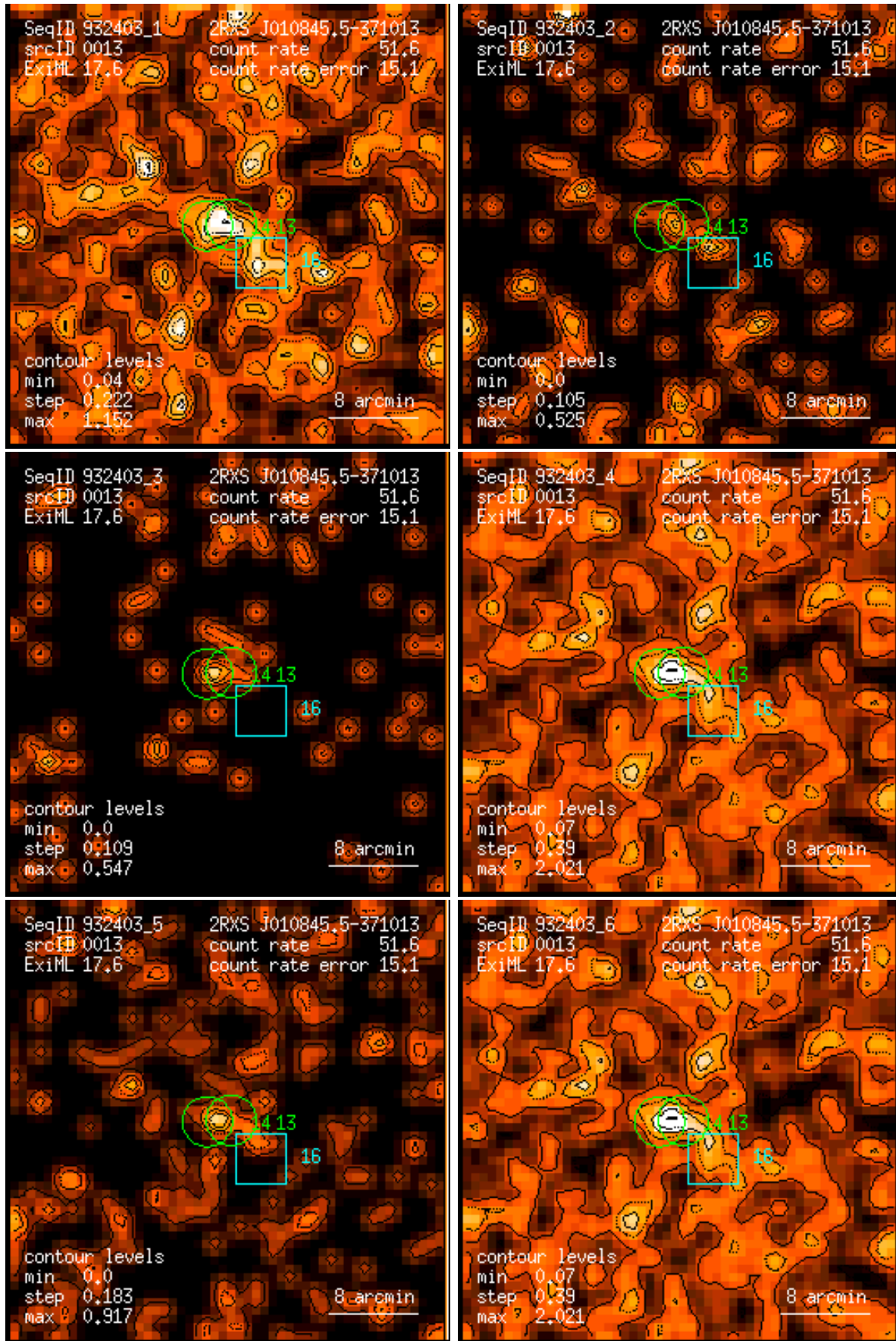
Figure 13: RASS 932403: detection 0013: band rate images, Gaussian filter: (1) PSPC channels 11 – 41, (2) 52 – 90, (3) 91 – 201, (4) 11 – 235, (5) 52 – 201, (6) 11 – 201. Broad band rates in counts/ks. Band rate contour levels in counts/ks/arcmin 2 .
