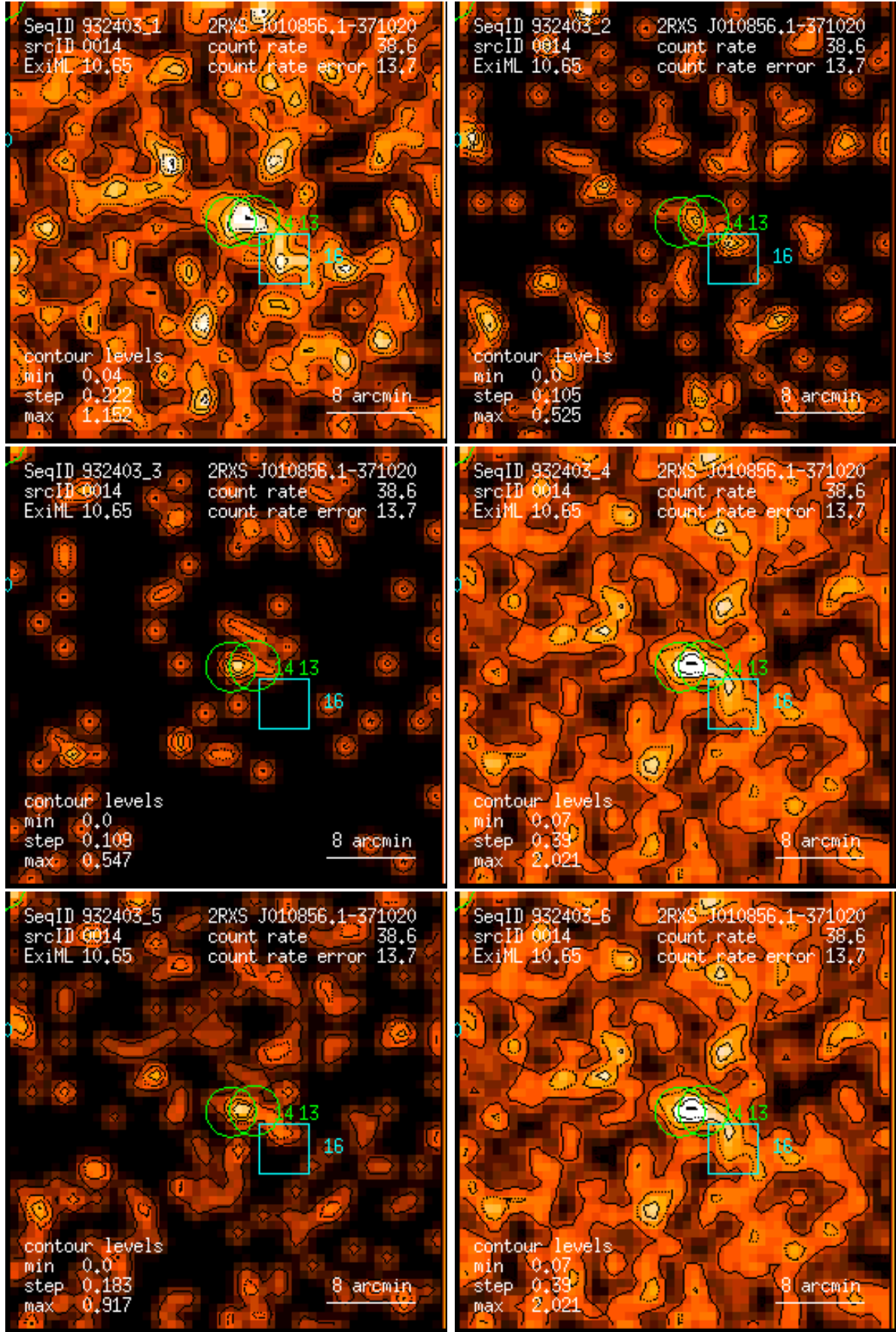
Figure 14: RASS 932403: detection 0014: band rate images, Gaussian filter: (1) PSPC channels 11 – 41, (2) 52 – 90, (3) 91 – 201, (4) 11 – 235, (5) 52 – 201, (6) 11 – 201. Broad band rates in counts/ks. Band rate contour levels in counts/ks/arcmin 2 .
