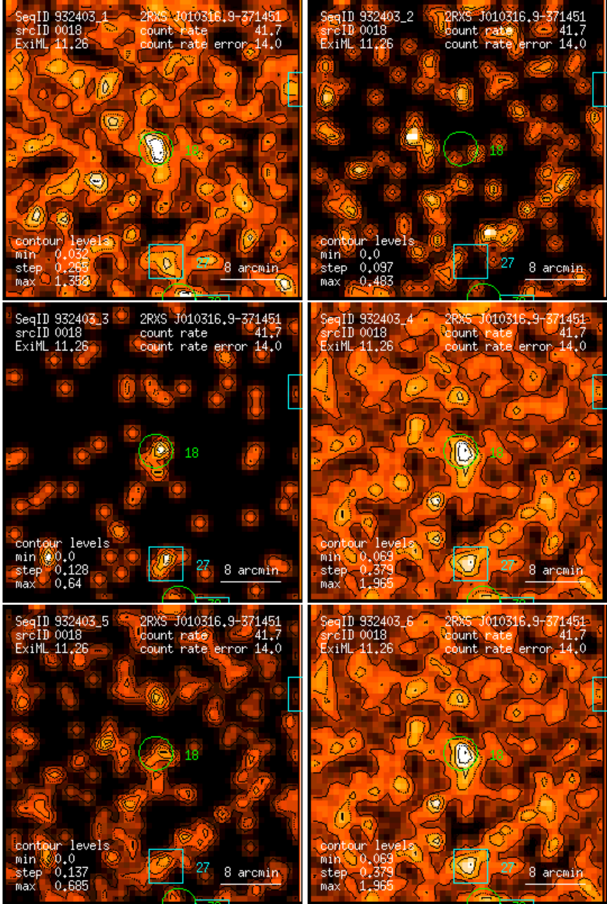
Figure 18: RASS 932403: detection 0018: band rate images, Gaussian filter: (1) PSPC channels 11 – 41, (2) 52 – 90, (3) 91 – 201, (4) 11 – 235, (5) 52 – 201, (6) 11 – 201. Broad band rates in counts/ks. Band rate contour levels in counts/ks/arcmin 2 .
