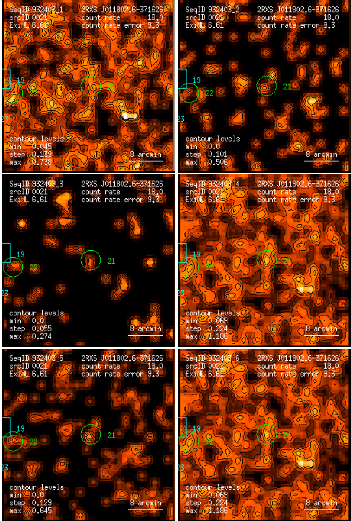
Figure 21: RASS 932403: detection 0021: band rate images, Gaussian filter: (1) PSPC channels 11 – 41, (2) 52 – 90, (3) 91 – 201, (4) 11 – 235, (5) 52 – 201, (6) 11 – 201. Broad band rates in counts/ks. Band rate contour levels in counts/ks/arcmin 2 .
