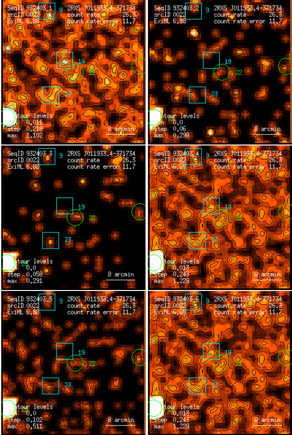
Figure 22: RASS 932403: detection 0022: band rate images, Gaussian filter: (1) PSPC channels 11 – 41, (2) 52 – 90, (3) 91 – 201, (4) 11 – 235, (5) 52 – 201, (6) 11 – 201. Broad band rates in counts/ks. Band rate contour levels in counts/ks/arcmin 2 .
