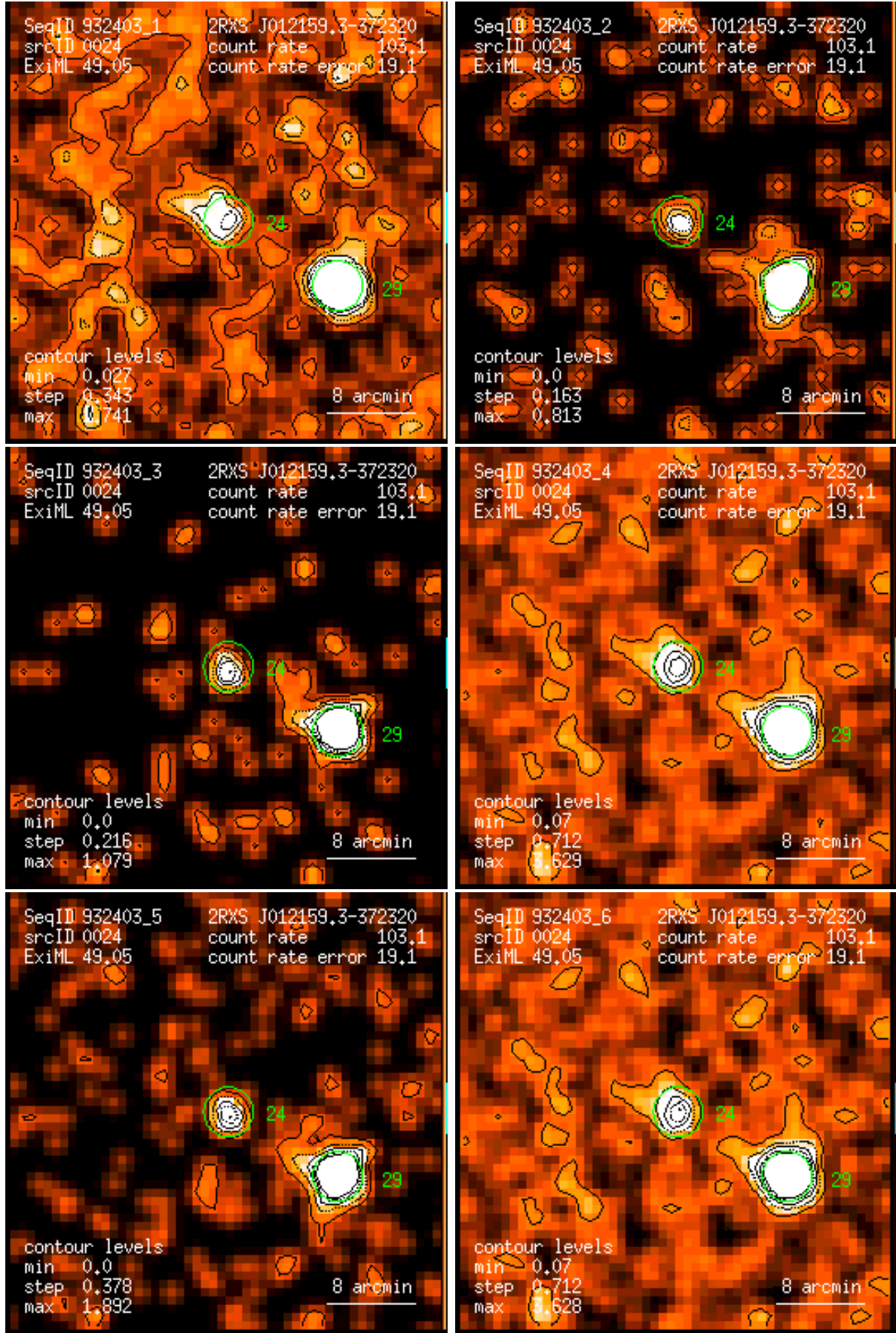
Figure 24: RASS 932403: detection 0024: band rate images, Gaussian filter: (1) PSPC channels 11 – 41, (2) 52 – 90, (3) 91 – 201, (4) 11 – 235, (5) 52 – 201, (6) 11 – 201. Broad band rates in counts/ks. Band rate contour levels in counts/ks/arcmin 2 .
