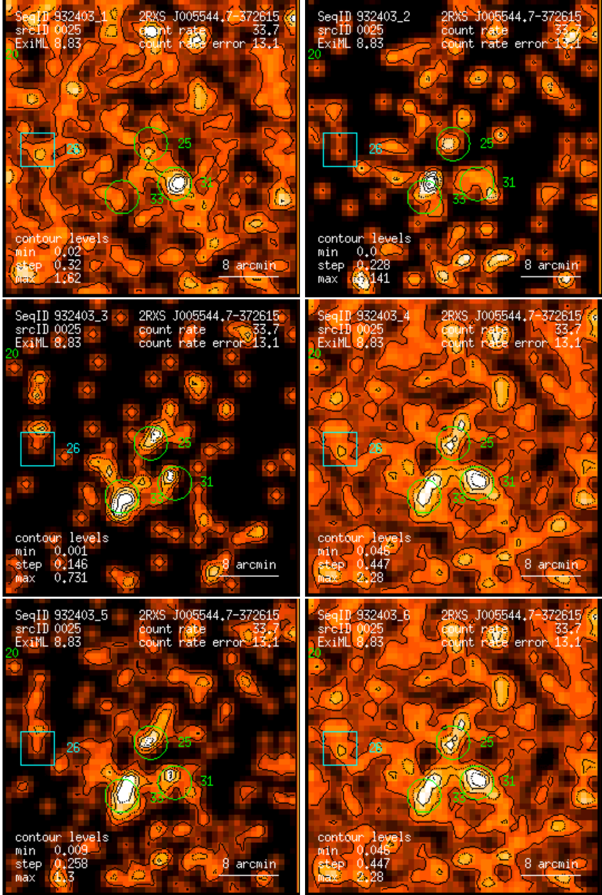
Figure 25: RASS 932403: detection 0025: band rate images, Gaussian filter: (1) PSPC channels 11 – 41, (2) 52 – 90, (3) 91 – 201, (4) 11 – 235, (5) 52 – 201, (6) 11 – 201. Broad band rates in counts/ks. Band rate contour levels in counts/ks/arcmin 2 .
