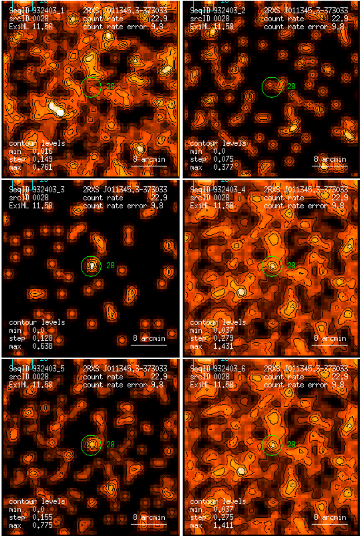
Figure 28: RASS 932403: detection 0028: band rate images, Gaussian filter: (1) PSPC channels 11 – 41, (2) 52 – 90, (3) 91 – 201, (4) 11 – 235, (5) 52 – 201, (6) 11 – 201. Broad band rates in counts/ks. Band rate contour levels in counts/ks/arcmin 2 .
