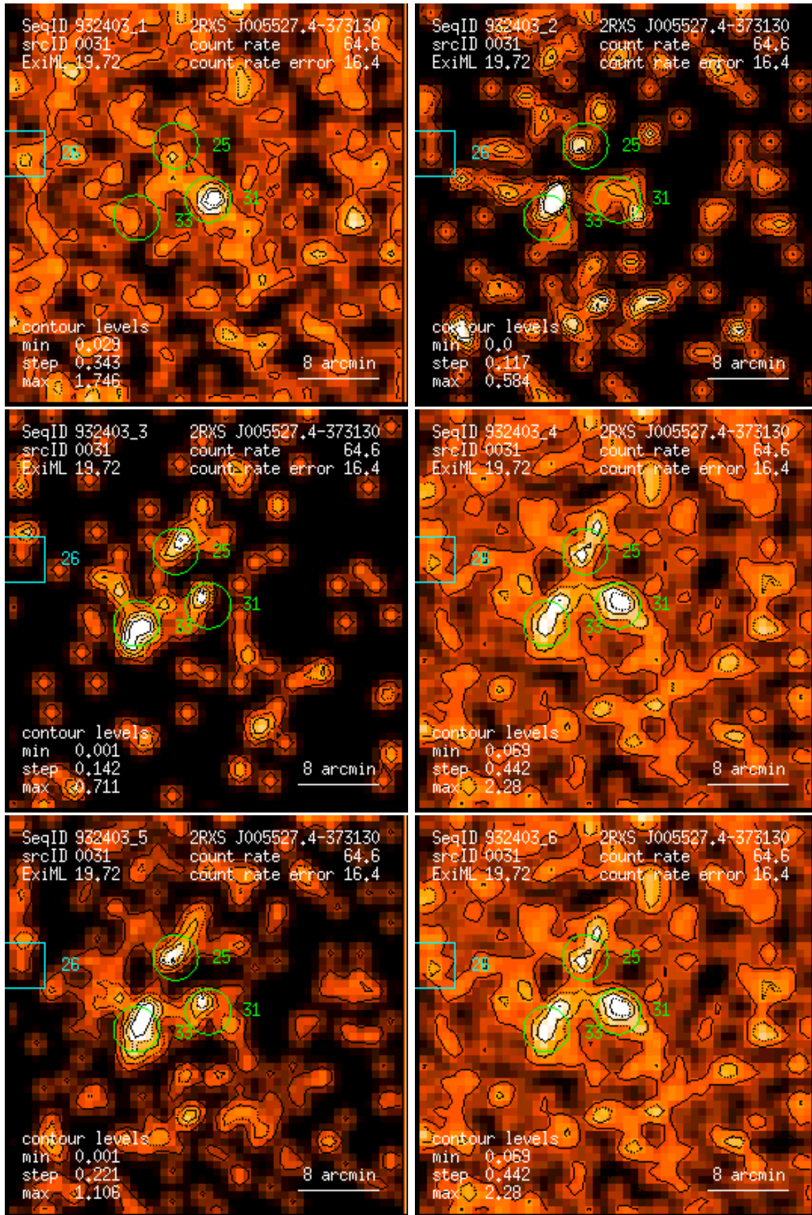
Figure 31: RASS 932403: detection 0031: band rate images, Gaussian filter: (1) PSPC channels 11 – 41, (2) 52 – 90, (3) 91 – 201, (4) 11 – 235, (5) 52 – 201, (6) 11 – 201. Broad band rates in counts/ks. Band rate contour levels in counts/ks/arcmin 2 .
