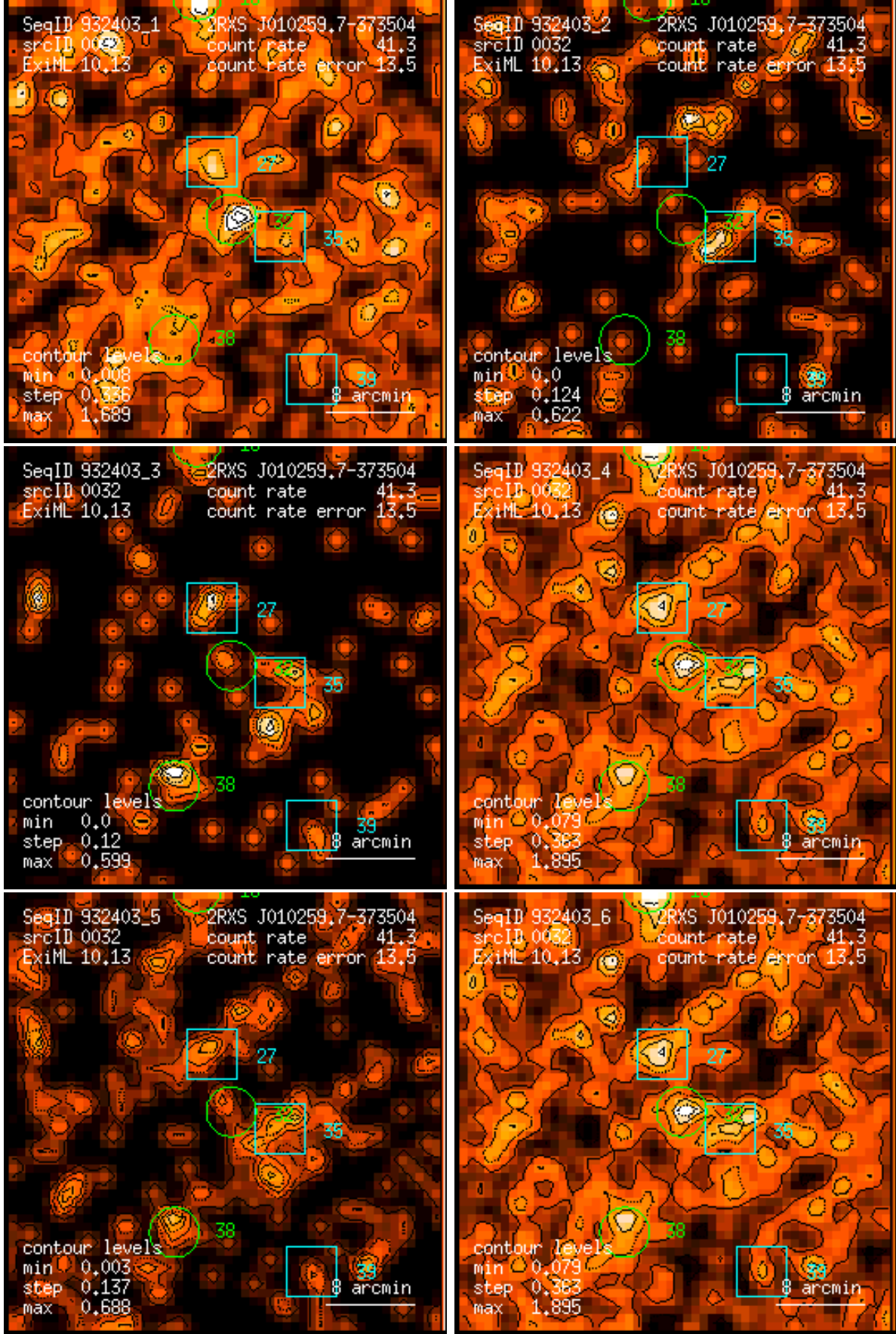
Figure 32: RASS 932403: detection 0032: band rate images, Gaussian filter: (1) PSPC channels 11 – 41, (2) 52 – 90, (3) 91 – 201, (4) 11 – 235, (5) 52 – 201, (6) 11 – 201. Broad band rates in counts/ks. Band rate contour levels in counts/ks/arcmin 2 .
