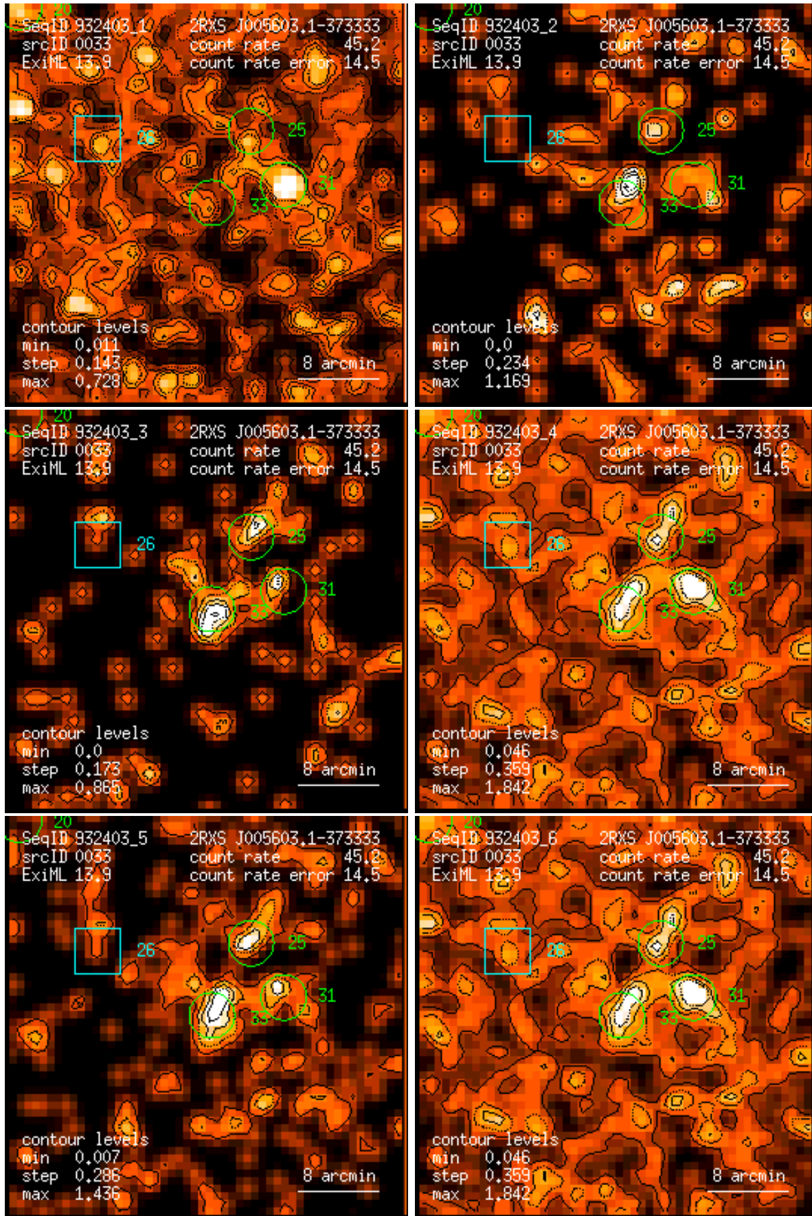
Figure 33: RASS 932403: detection 0033: band rate images, Gaussian filter: (1) PSPC channels 11 – 41, (2) 52 – 90, (3) 91 – 201, (4) 11 – 235, (5) 52 – 201, (6) 11 – 201. Broad band rates in counts/ks. Band rate contour levels in counts/ks/arcmin 2 .
