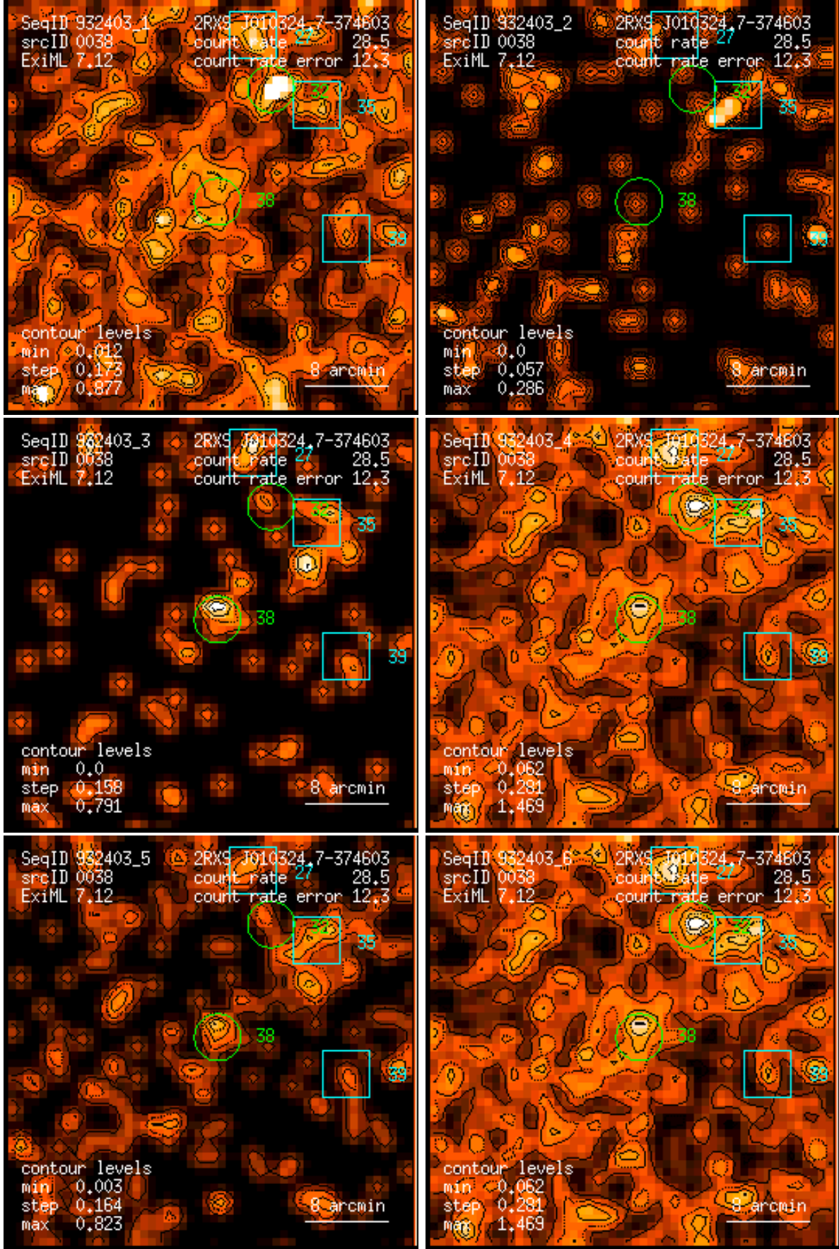
Figure 38: RASS 932403: detection 0038: band rate images, Gaussian filter: (1) PSPC channels 11 – 41, (2) 52 – 90, (3) 91 – 201, (4) 11 – 235, (5) 52 – 201, (6) 11 – 201. Broad band rates in counts/ks. Band rate contour levels in counts/ks/arcmin 2 .
