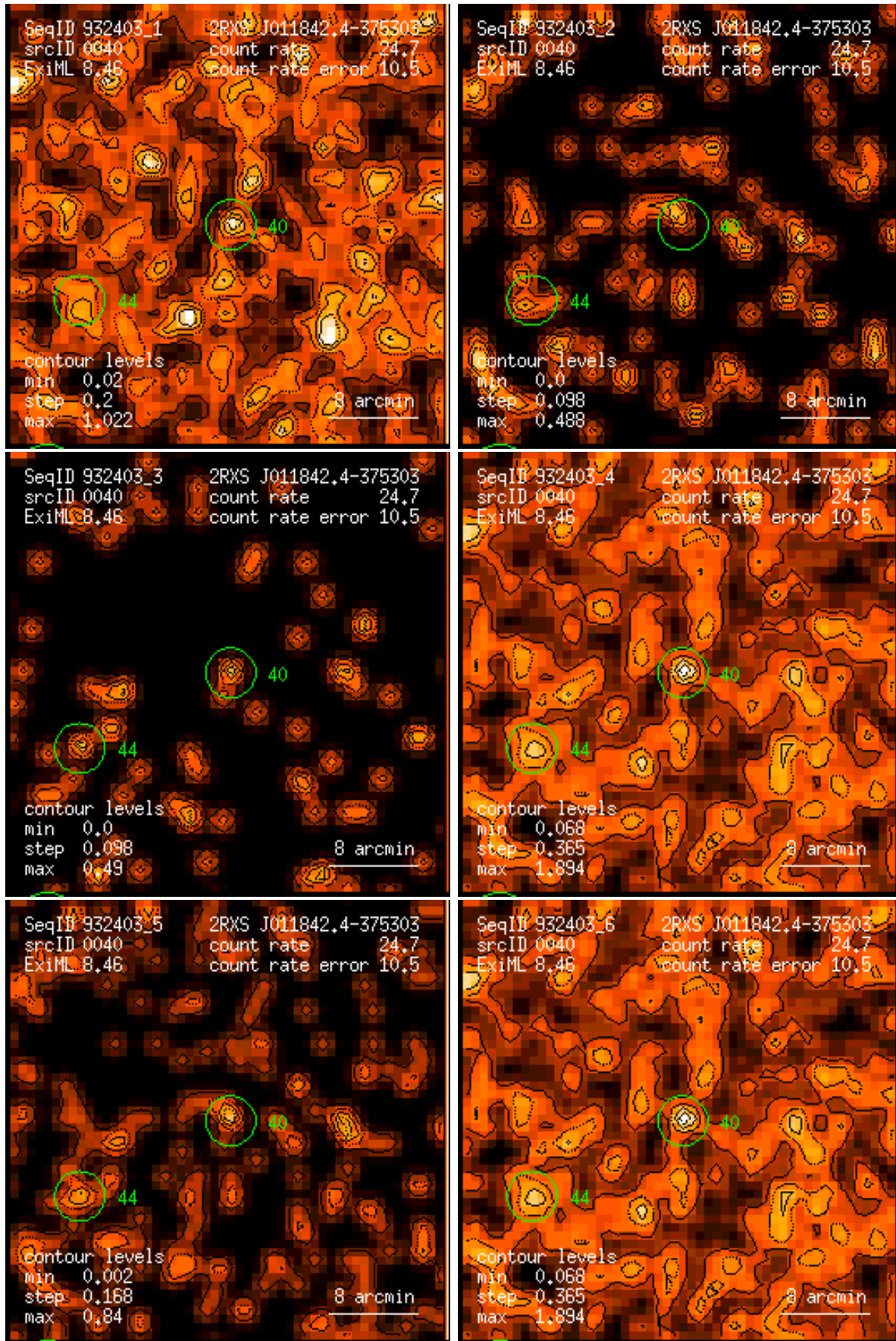
Figure 40: RASS 932403: detection 0040: band rate images, Gaussian filter: (1) PSPC channels 11 – 41, (2) 52 – 90, (3) 91 – 201, (4) 11 – 235, (5) 52 – 201, (6) 11 – 201. Broad band rates in counts/ks. Band rate contour levels in counts/ks/arcmin 2 .
