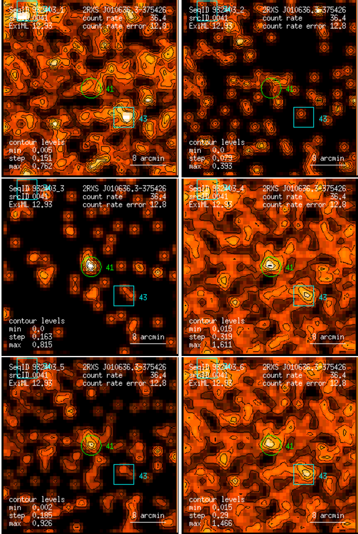
Figure 41: RASS 932403: detection 0041: band rate images, Gaussian filter: (1) PSPC channels 11 – 41, (2) 52 – 90, (3) 91 – 201, (4) 11 – 235, (5) 52 – 201, (6) 11 – 201. Broad band rates in counts/ks. Band rate contour levels in counts/ks/arcmin 2 .
