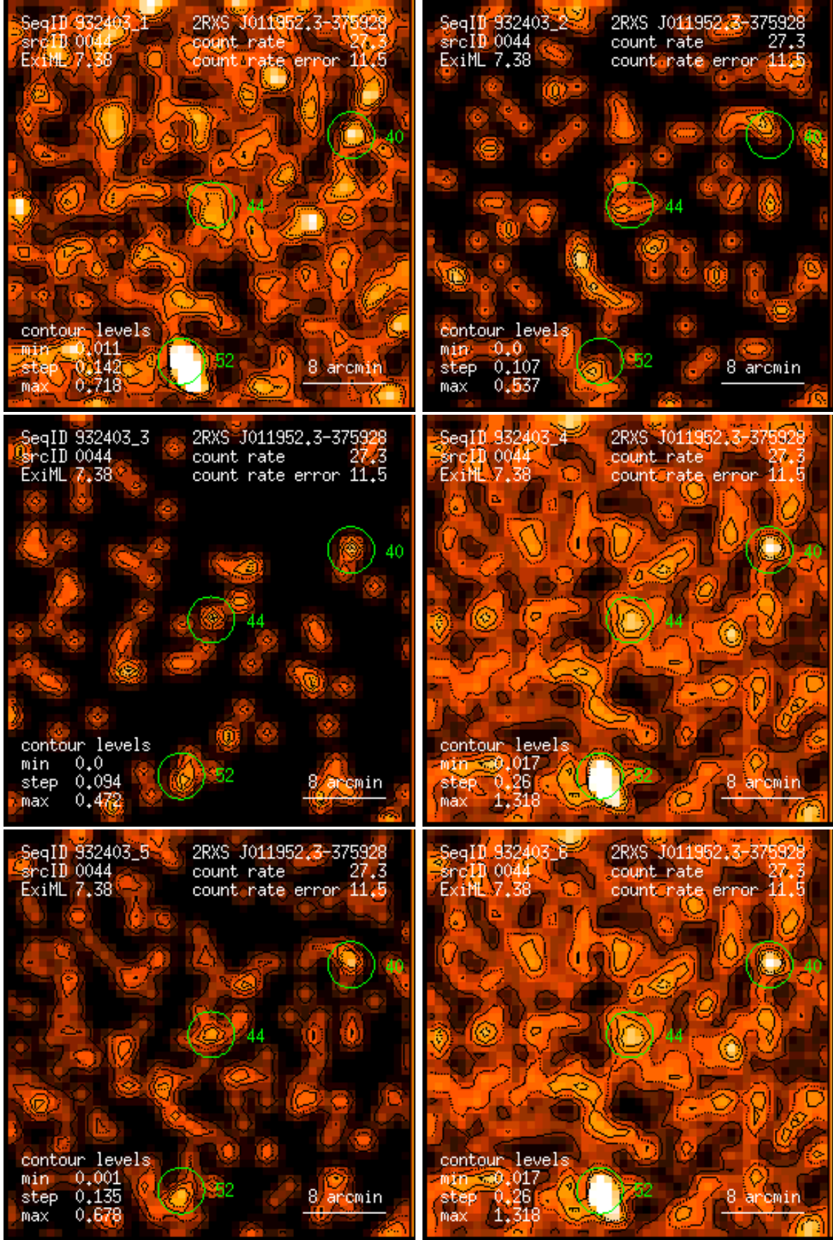
Figure 44: RASS 932403: detection 0044: band rate images, Gaussian filter: (1) PSPC channels 11 – 41, (2) 52 – 90, (3) 91 – 201, (4) 11 – 235, (5) 52 – 201, (6) 11 – 201. Broad band rates in counts/ks. Band rate contour levels in counts/ks/arcmin 2 .
