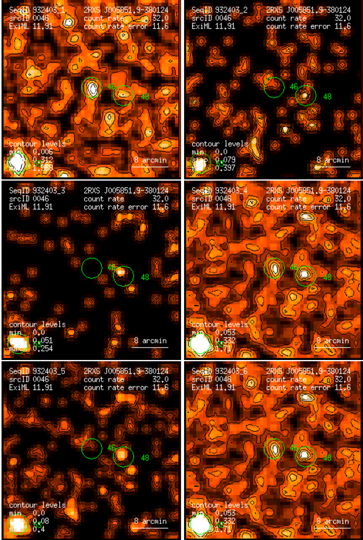
Figure 46: RASS 932403: detection 0046: band rate images, Gaussian filter: (1) PSPC channels 11 – 41, (2) 52 – 90, (3) 91 – 201, (4) 11 – 235, (5) 52 – 201, (6) 11 – 201. Broad band rates in counts/ks. Band rate contour levels in counts/ks/arcmin 2 .
