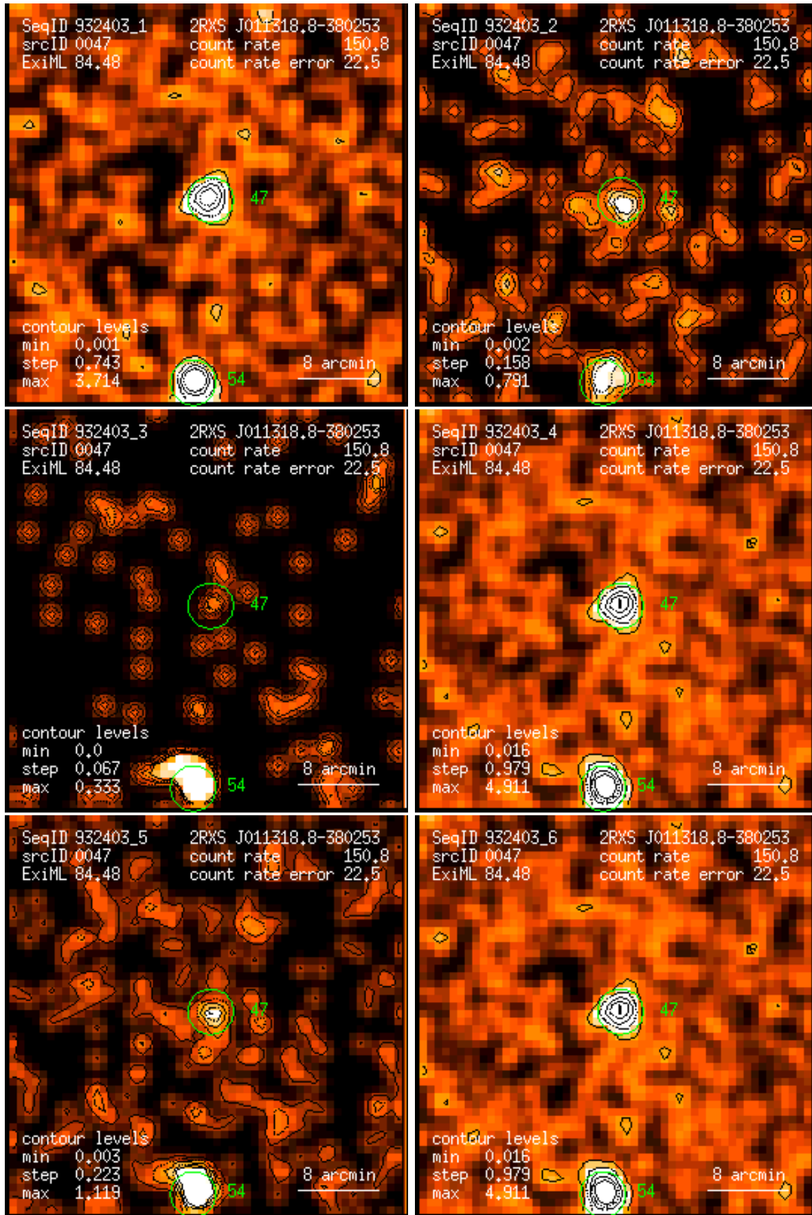
Figure 47: RASS 932403: detection 0047: band rate images, Gaussian filter: (1) PSPC channels 11 – 41, (2) 52 – 90, (3) 91 – 201, (4) 11 – 235, (5) 52 – 201, (6) 11 – 201. Broad band rates in counts/ks. Band rate contour levels in counts/ks/arcmin 2 .
