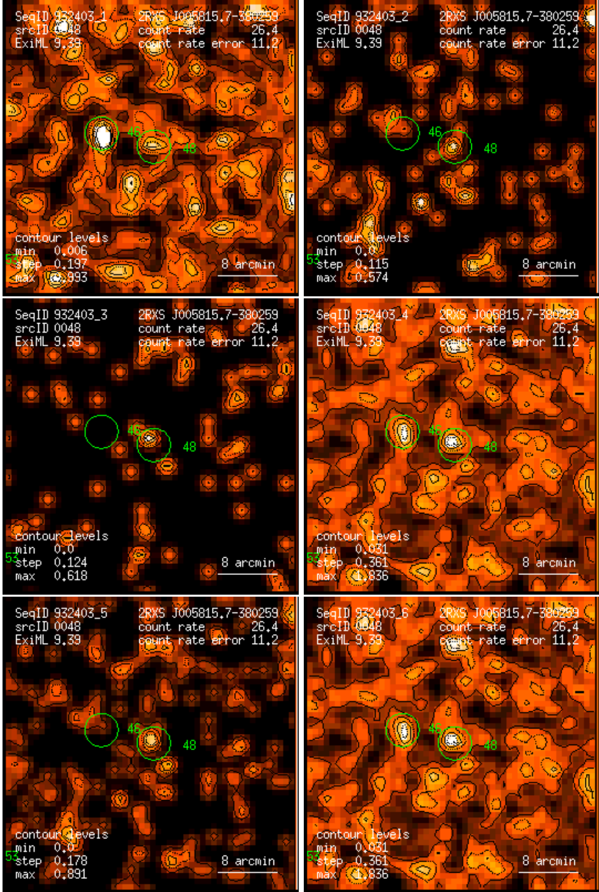
Figure 48: RASS 932403: detection 0048: band rate images, Gaussian filter: (1) PSPC channels 11 – 41, (2) 52 – 90, (3) 91 – 201, (4) 11 – 235, (5) 52 – 201, (6) 11 – 201. Broad band rates in counts/ks. Band rate contour levels in counts/ks/arcmin 2 .
