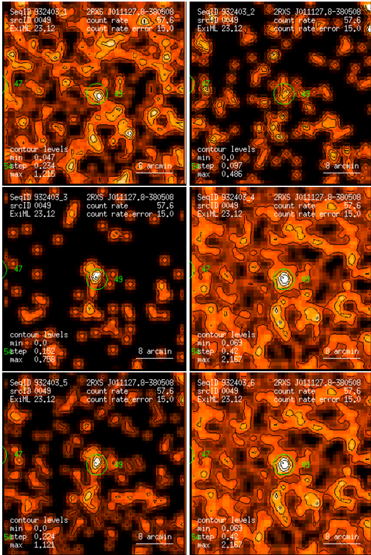
Figure 49: RASS 932403: detection 0049: band rate images, Gaussian filter: (1) PSPC channels 11 – 41, (2) 52 – 90, (3) 91 – 201, (4) 11 – 235, (5) 52 – 201, (6) 11 – 201. Broad band rates in counts/ks. Band rate contour levels in counts/ks/arcmin 2 .
