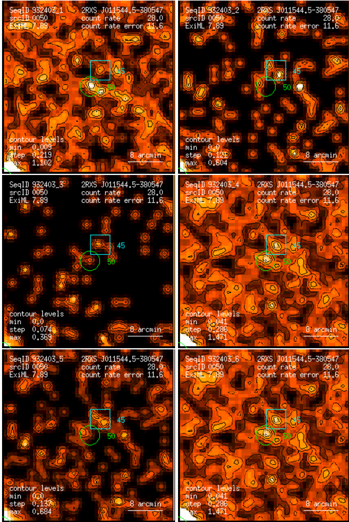
Figure 50: RASS 932403: detection 0050: band rate images, Gaussian filter: (1) PSPC channels 11 – 41, (2) 52 – 90, (3) 91 – 201, (4) 11 – 235, (5) 52 – 201, (6) 11 – 201. Broad band rates in counts/ks. Band rate contour levels in counts/ks/arcmin 2 .
