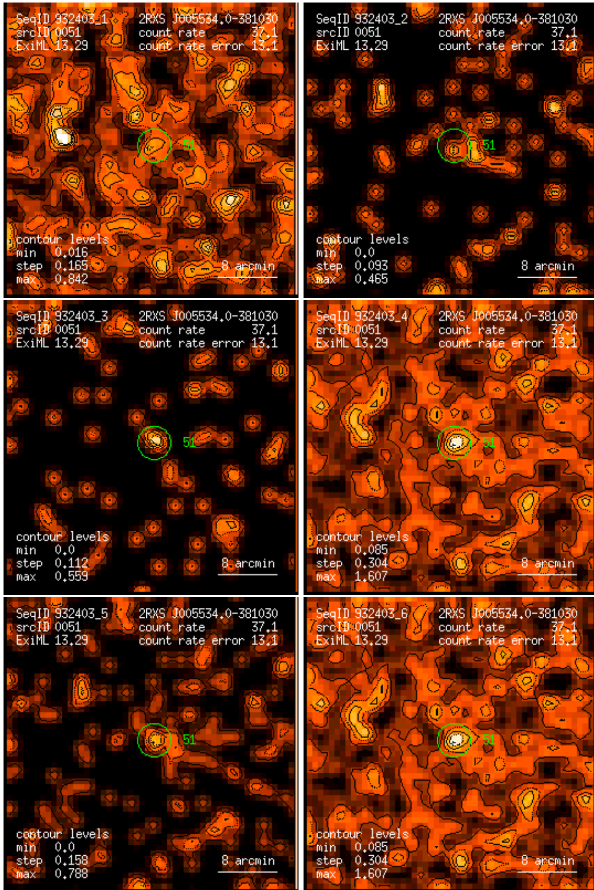
Figure 51: RASS 932403: detection 0051: band rate images, Gaussian filter: (1) PSPC channels 11 – 41, (2) 52 – 90, (3) 91 – 201, (4) 11 – 235, (5) 52 – 201, (6) 11 – 201. Broad band rates in counts/ks. Band rate contour levels in counts/ks/arcmin 2 .
