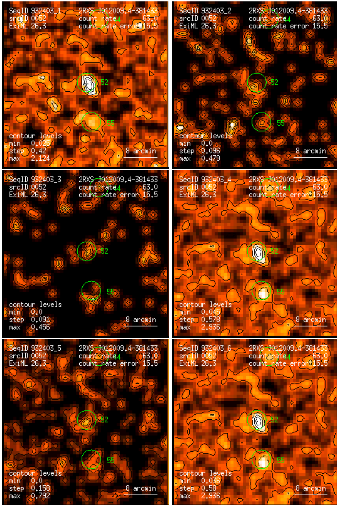
Figure 52: RASS 932403: detection 0052: band rate images, Gaussian filter: (1) PSPC channels 11 – 41, (2) 52 – 90, (3) 91 – 201, (4) 11 – 235, (5) 52 – 201, (6) 11 – 201. Broad band rates in counts/ks. Band rate contour levels in counts/ks/arcmin 2 .
