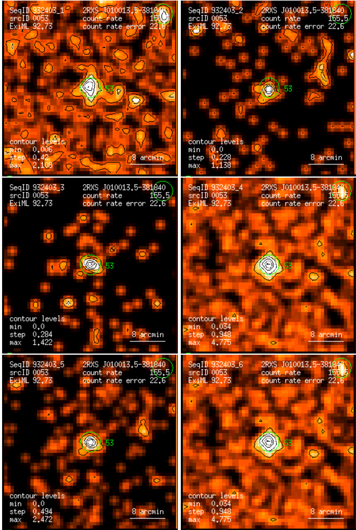
Figure 53: RASS 932403: detection 0053: band rate images, Gaussian filter: (1) PSPC channels 11 – 41, (2) 52 – 90, (3) 91 – 201, (4) 11 – 235, (5) 52 – 201, (6) 11 – 201. Broad band rates in counts/ks. Band rate contour levels in counts/ks/arcmin 2 .
