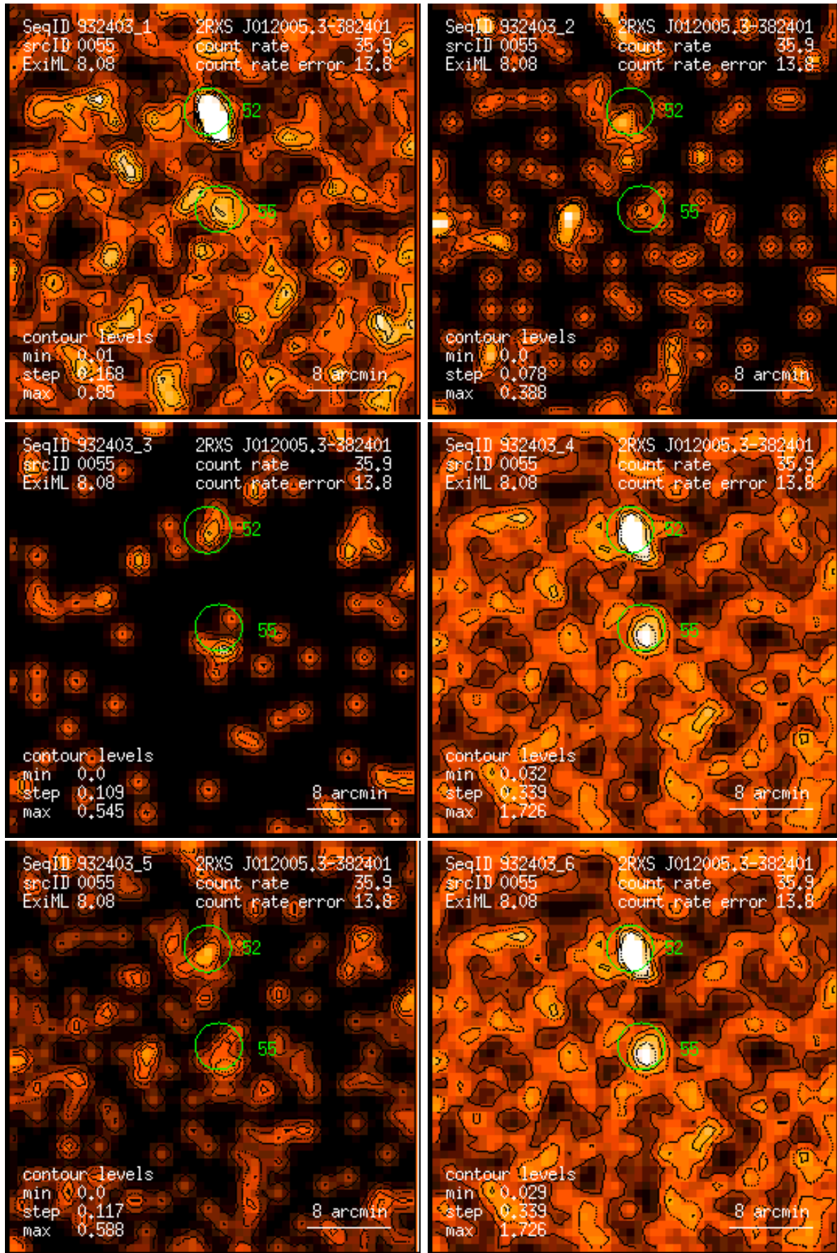
Figure 55: RASS 932403: detection 0055: band rate images, Gaussian filter: (1) PSPC channels 11 – 41, (2) 52 – 90, (3) 91 – 201, (4) 11 – 235, (5) 52 – 201, (6) 11 – 201. Broad band rates in counts/ks. Band rate contour levels in counts/ks/arcmin 2 .
