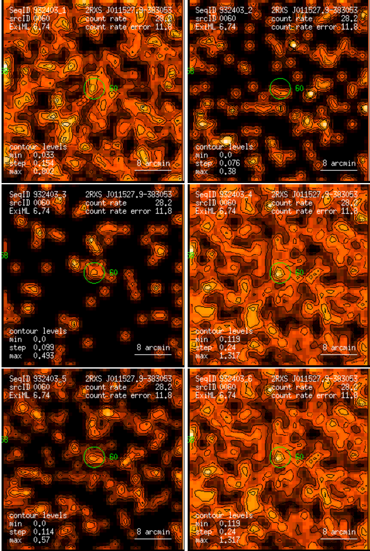
Figure 60: RASS 932403: detection 0060: band rate images, Gaussian filter: (1) PSPC channels 11 – 41, (2) 52 – 90, (3) 91 – 201, (4) 11 – 235, (5) 52 – 201, (6) 11 – 201. Broad band rates in counts/ks. Band rate contour levels in counts/ks/arcmin 2 .
