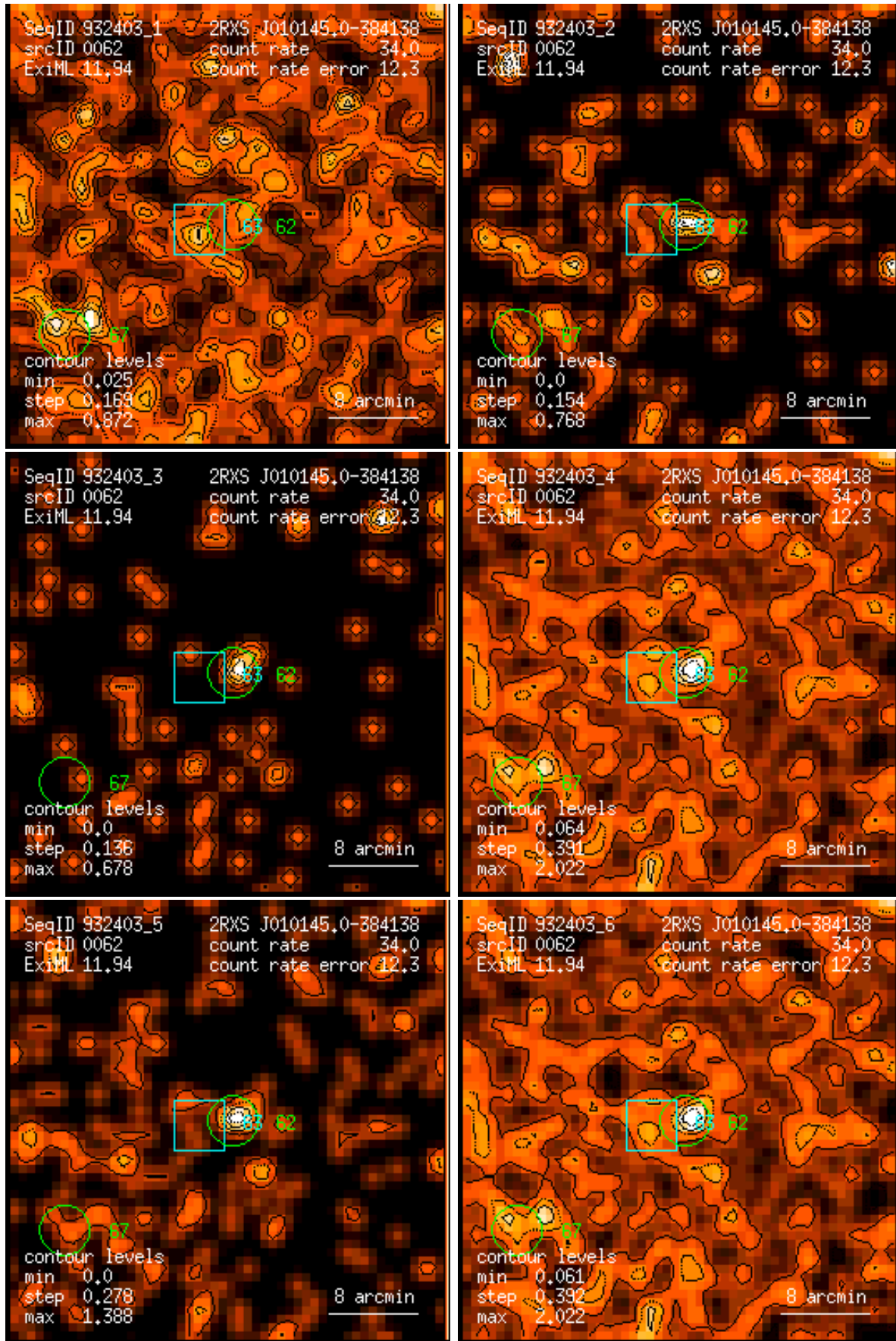
Figure 62: RASS 932403: detection 0062: band rate images, Gaussian filter: (1) PSPC channels 11 – 41, (2) 52 – 90, (3) 91 – 201, (4) 11 – 235, (5) 52 – 201, (6) 11 – 201. Broad band rates in counts/ks. Band rate contour levels in counts/ks/arcmin 2 .
