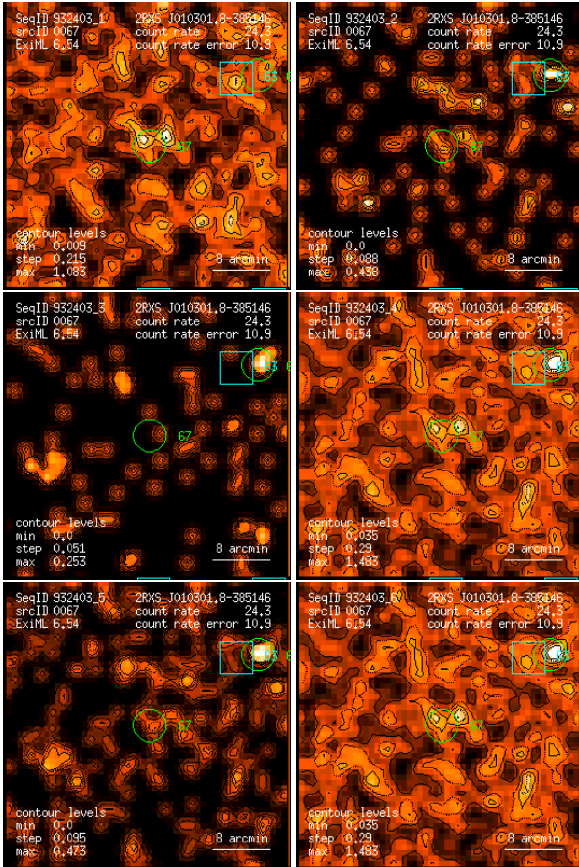
Figure 67: RASS 932403: detection 0067: band rate images, Gaussian filter: (1) PSPC channels 11 – 41, (2) 52 – 90, (3) 91 – 201, (4) 11 – 235, (5) 52 – 201, (6) 11 – 201. Broad band rates in counts/ks. Band rate contour levels in counts/ks/arcmin 2 .
