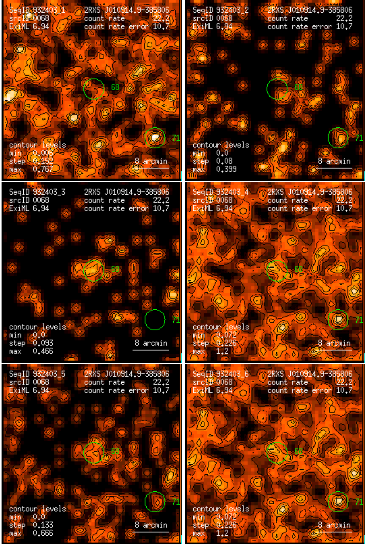
Figure 68: RASS 932403: detection 0068: band rate images, Gaussian filter: (1) PSPC channels 11 – 41, (2) 52 – 90, (3) 91 – 201, (4) 11 – 235, (5) 52 – 201, (6) 11 – 201. Broad band rates in counts/ks. Band rate contour levels in counts/ks/arcmin 2 .
