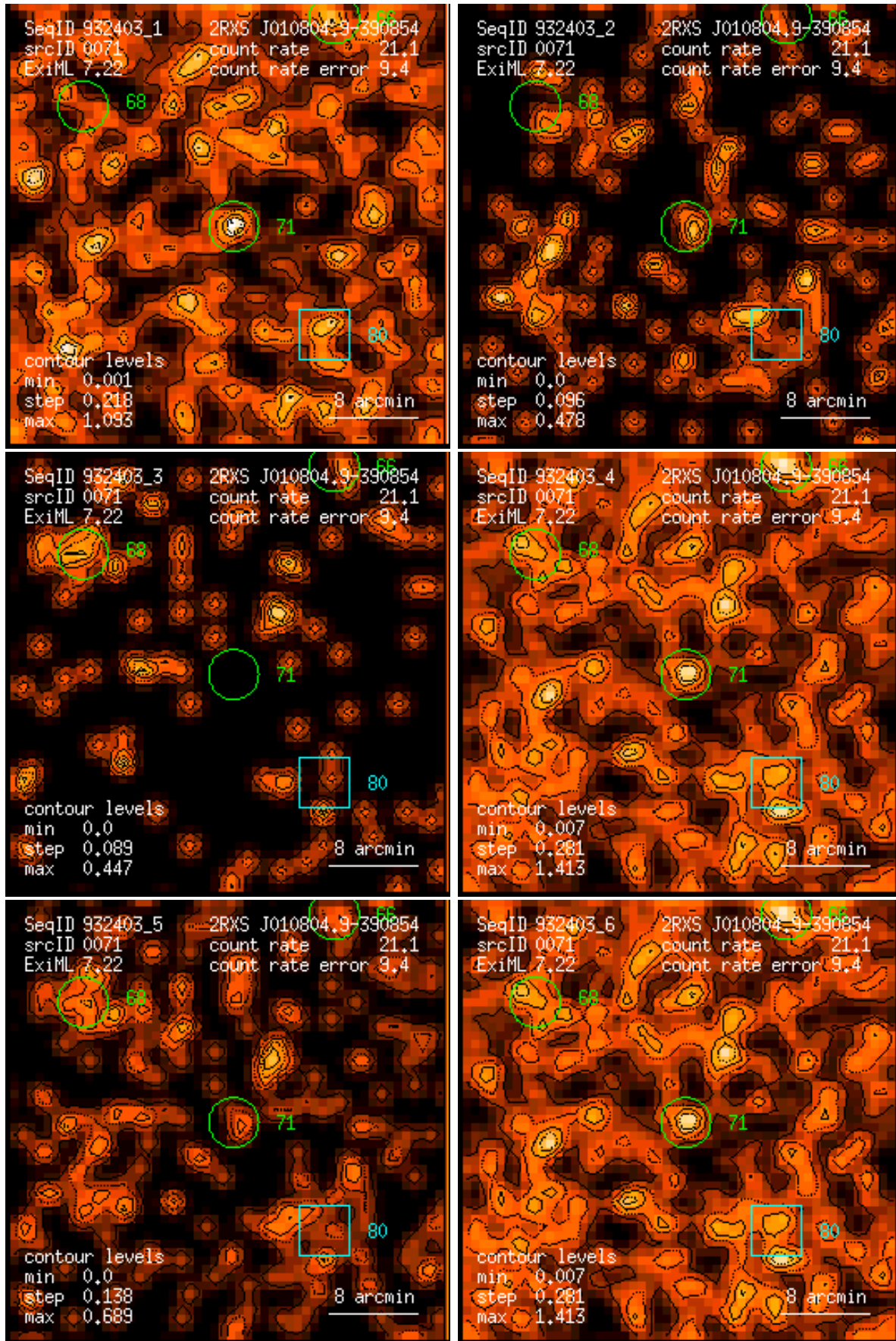
Figure 71: RASS 932403: detection 0071: band rate images, Gaussian filter: (1) PSPC channels 11 – 41, (2) 52 – 90, (3) 91 – 201, (4) 11 – 235, (5) 52 – 201, (6) 11 – 201. Broad band rates in counts/ks. Band rate contour levels in counts/ks/arcmin 2 .
