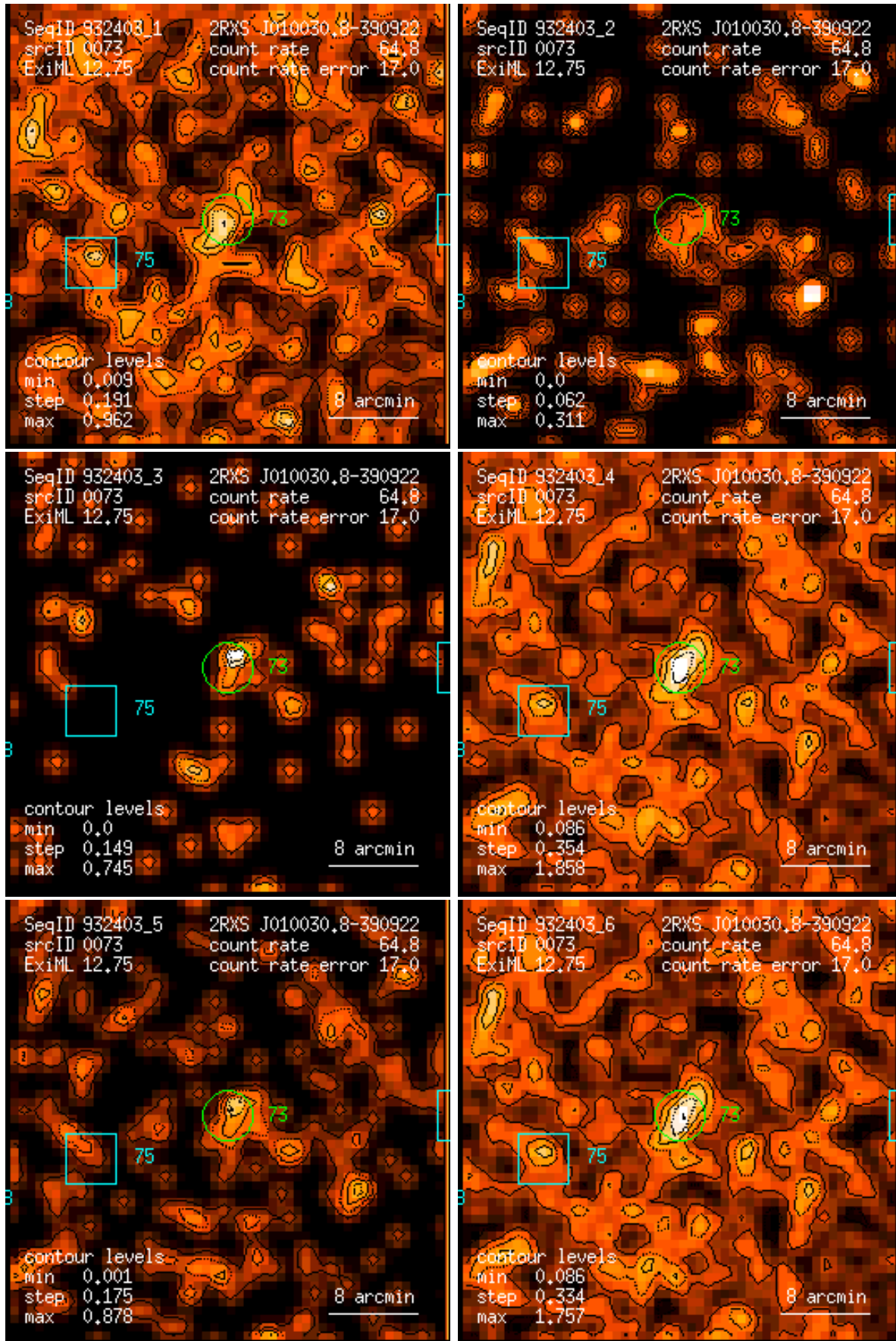
Figure 73: RASS 932403: detection 0073: band rate images, Gaussian filter: (1) PSPC channels 11 – 41, (2) 52 – 90, (3) 91 – 201, (4) 11 – 235, (5) 52 – 201, (6) 11 – 201. Broad band rates in counts/ks. Band rate contour levels in counts/ks/arcmin 2 .
